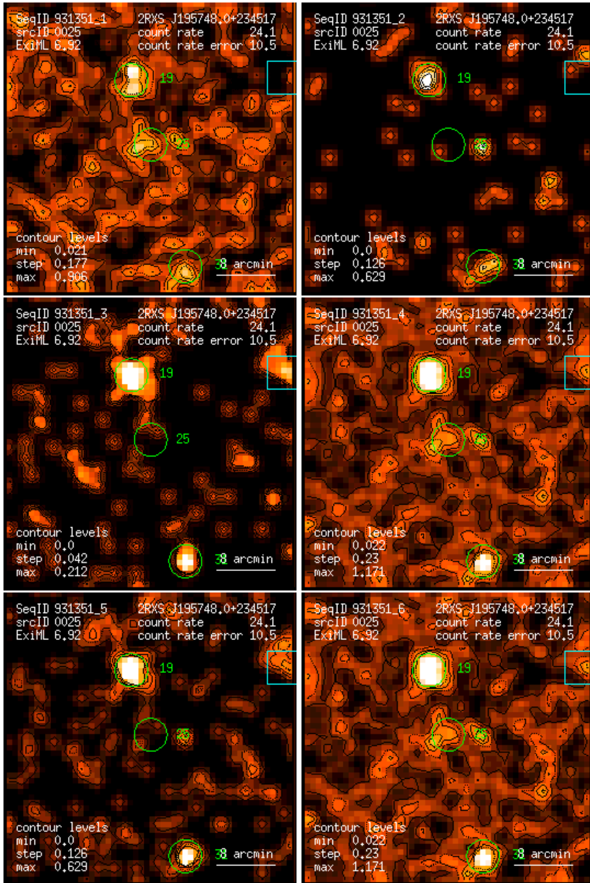
Figure 25: RASS 931351: detection 0025: band rate images, Gaussian filter: (1) PSPC channels 11 – 41, (2) 52 – 90, (3) 91 – 201, (4) 11 – 235, (5) 52 – 201, (6) 11 – 201. Broad band rates in counts/ks. Band rate contour levels in counts/ks/arcmin 2 .
