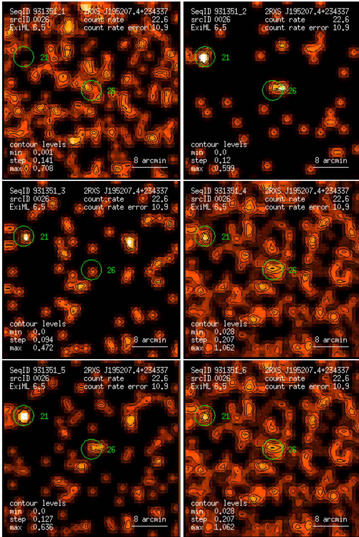
Figure 26: RASS 931351: detection 0026: band rate images, Gaussian filter: (1) PSPC channels 11 – 41, (2) 52 – 90, (3) 91 – 201, (4) 11 – 235, (5) 52 – 201, (6) 11 – 201. Broad band rates in counts/ks. Band rate contour levels in counts/ks/arcmin 2 .
