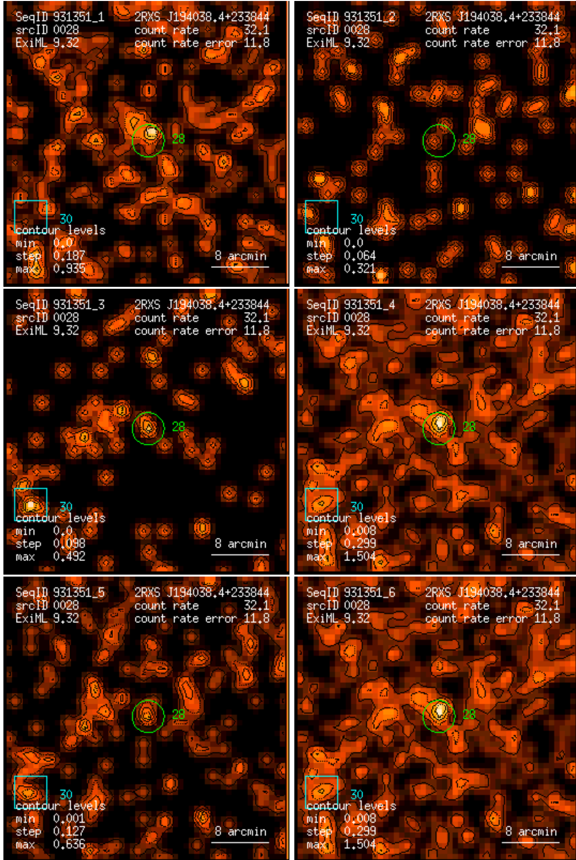
Figure 28: RASS 931351: detection 0028: band rate images, Gaussian filter: (1) PSPC channels 11 – 41, (2) 52 – 90, (3) 91 – 201, (4) 11 – 235, (5) 52 – 201, (6) 11 – 201. Broad band rates in counts/ks. Band rate contour levels in counts/ks/arcmin 2 .
