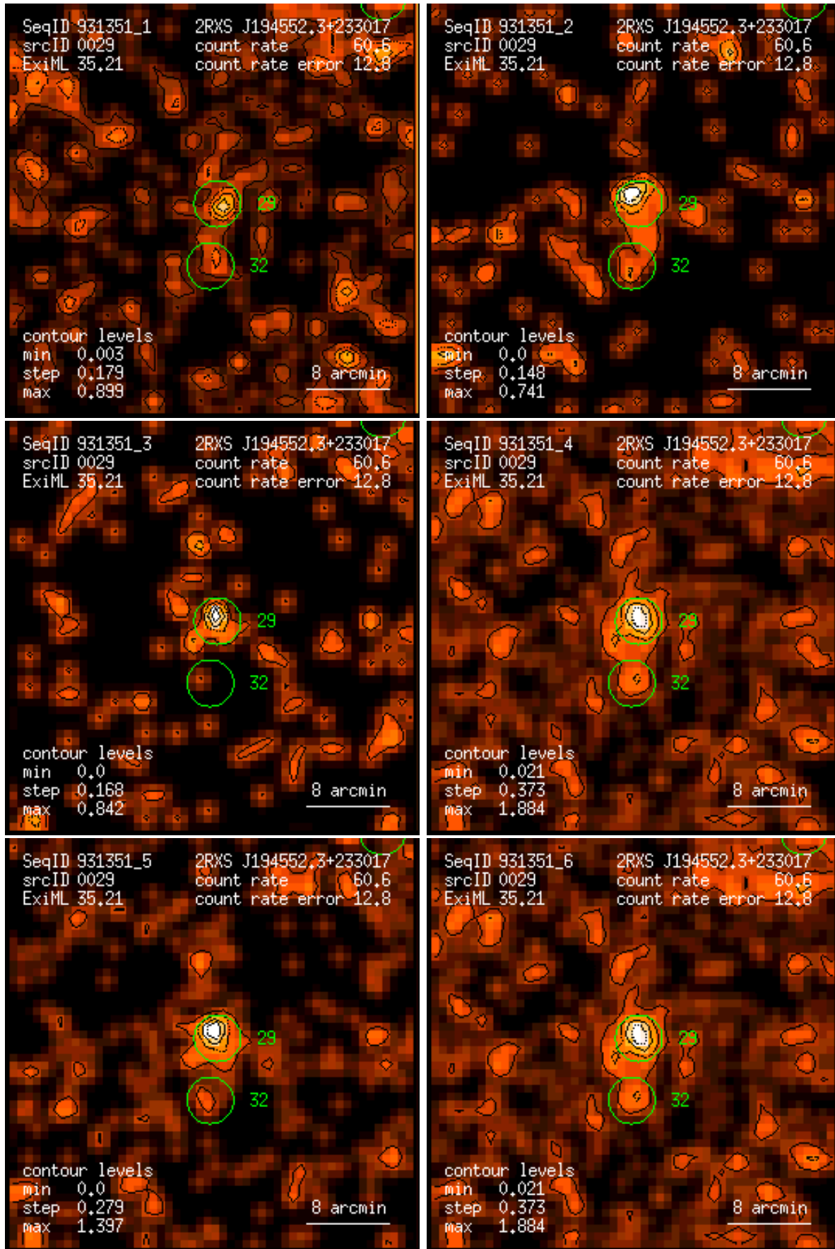
Figure 29: RASS 931351: detection 0029: band rate images, Gaussian filter: (1) PSPC channels 11 – 41, (2) 52 – 90, (3) 91 – 201, (4) 11 – 235, (5) 52 – 201, (6) 11 – 201. Broad band rates in counts/ks. Band rate contour levels in counts/ks/arcmin 2 .
