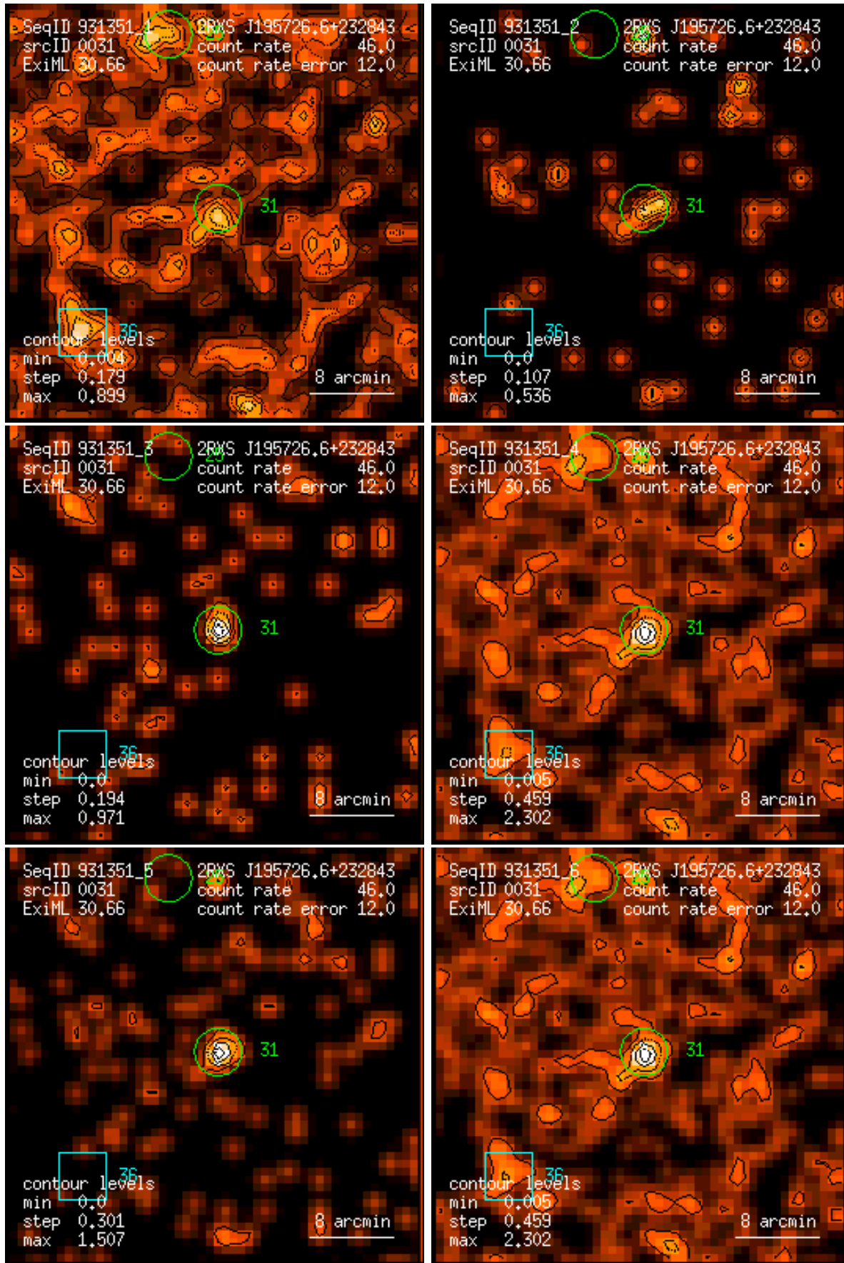
Figure 31: RASS 931351: detection 0031: band rate images, Gaussian filter: (1) PSPC channels 11 – 41, (2) 52 – 90, (3) 91 – 201, (4) 11 – 235, (5) 52 – 201, (6) 11 – 201. Broad band rates in counts/ks. Band rate contour levels in counts/ks/arcmin 2 .
