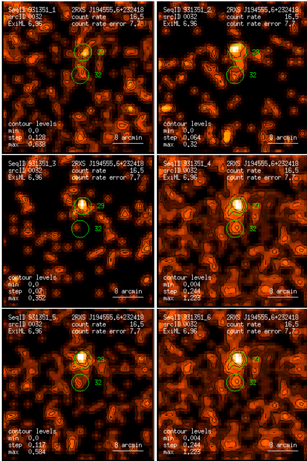
Figure 32: RASS 931351: detection 0032: band rate images, Gaussian filter: (1) PSPC channels 11 – 41, (2) 52 – 90, (3) 91 – 201, (4) 11 – 235, (5) 52 – 201, (6) 11 – 201. Broad band rates in counts/ks. Band rate contour levels in counts/ks/arcmin 2 .
