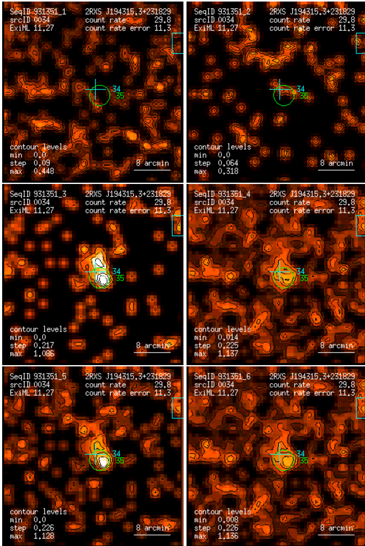
Figure 34: RASS 931351: detection 0034: band rate images, Gaussian filter: (1) PSPC channels 11 – 41, (2) 52 – 90, (3) 91 – 201, (4) 11 – 235, (5) 52 – 201, (6) 11 – 201. Broad band rates in counts/ks. Band rate contour levels in counts/ks/arcmin 2 .
