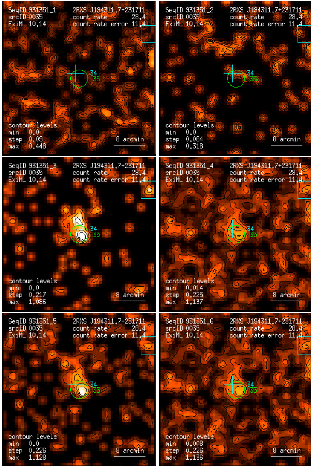
Figure 35: RASS 931351: detection 0035: band rate images, Gaussian filter: (1) PSPC channels 11 – 41, (2) 52 – 90, (3) 91 – 201, (4) 11 – 235, (5) 52 – 201, (6) 11 – 201. Broad band rates in counts/ks. Band rate contour levels in counts/ks/arcmin 2 .
