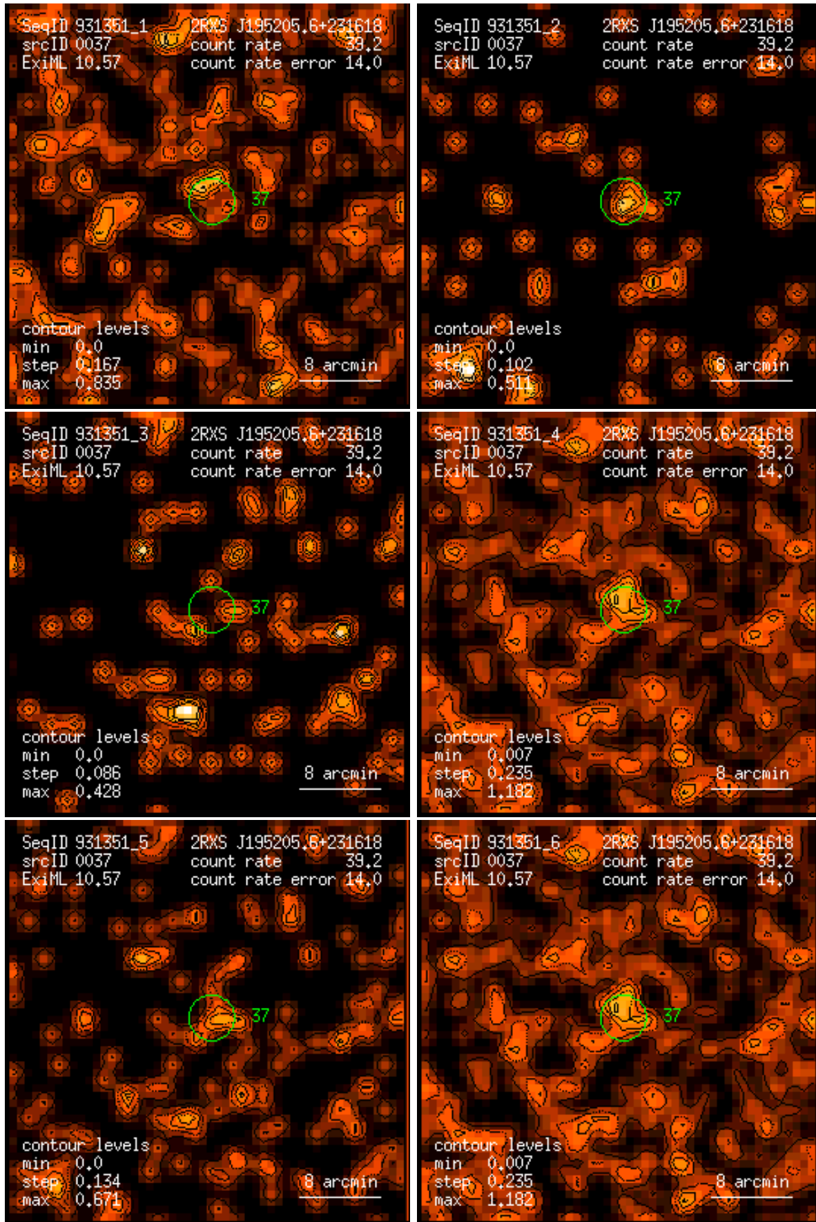
Figure 37: RASS 931351: detection 0037: band rate images, Gaussian filter: (1) PSPC channels 11 – 41, (2) 52 – 90, (3) 91 – 201, (4) 11 – 235, (5) 52 – 201, (6) 11 – 201. Broad band rates in counts/ks. Band rate contour levels in counts/ks/arcmin 2 .
