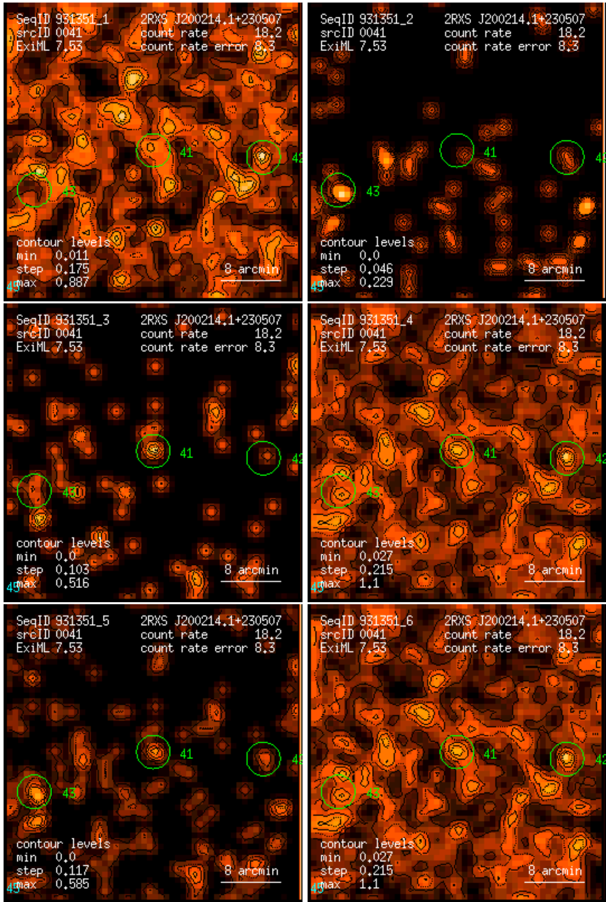
Figure 41: RASS 931351: detection 0041: band rate images, Gaussian filter: (1) PSPC channels 11 – 41, (2) 52 – 90, (3) 91 – 201, (4) 11 – 235, (5) 52 – 201, (6) 11 – 201. Broad band rates in counts/ks. Band rate contour levels in counts/ks/arcmin 2 .
