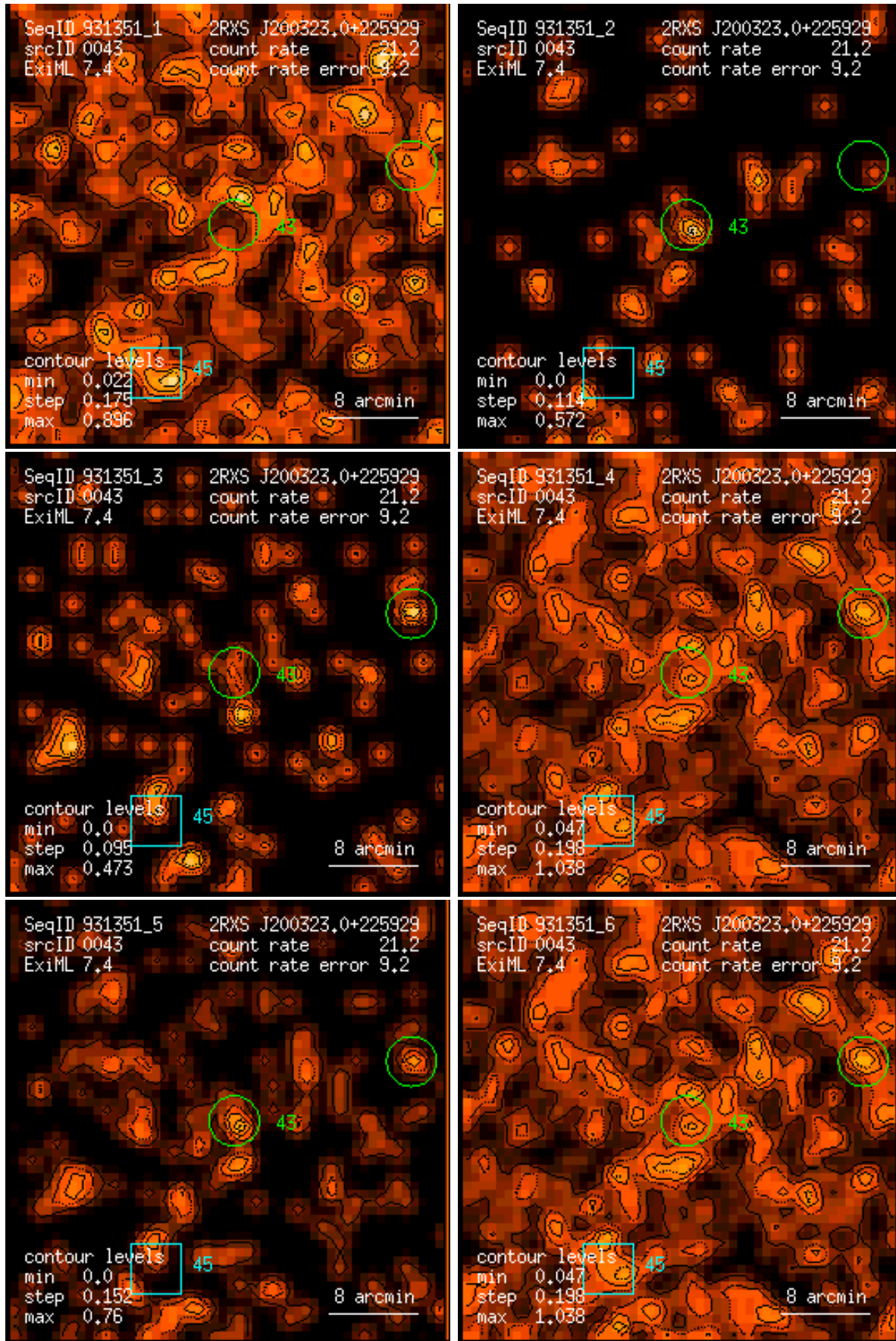
Figure 43: RASS 931351: detection 0043: band rate images, Gaussian filter: (1) PSPC channels 11 – 41, (2) 52 – 90, (3) 91 – 201, (4) 11 – 235, (5) 52 – 201, (6) 11 – 201. Broad band rates in counts/ks. Band rate contour levels in counts/ks/arcmin 2 .
