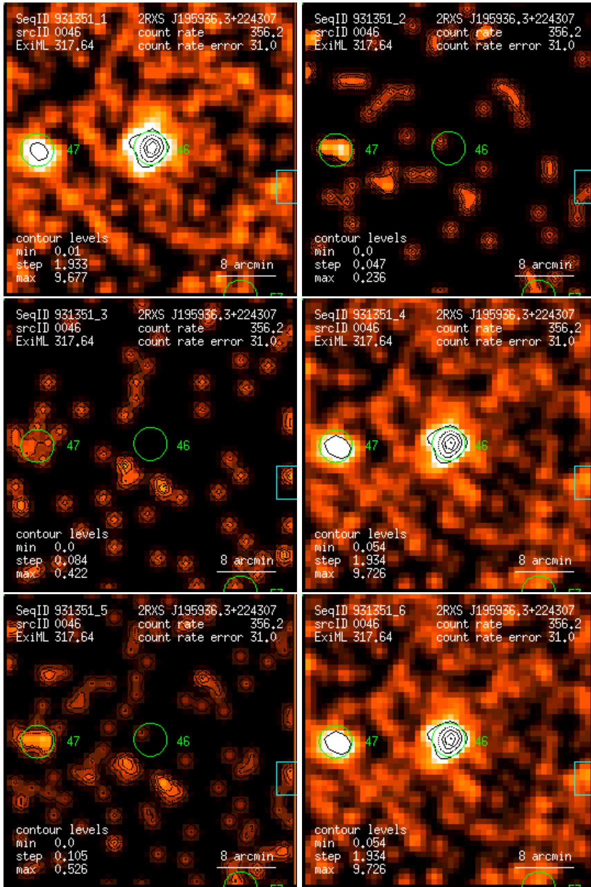
Figure 46: RASS 931351: detection 0046: band rate images, Gaussian filter: (1) PSPC channels 11 – 41, (2) 52 – 90, (3) 91 – 201, (4) 11 – 235, (5) 52 – 201, (6) 11 – 201. Broad band rates in counts/ks. Band rate contour levels in counts/ks/arcmin 2 .
