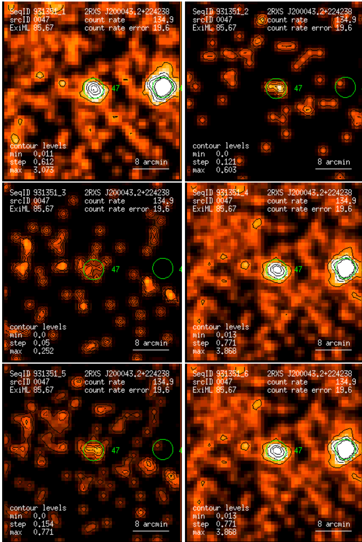
Figure 47: RASS 931351: detection 0047: band rate images, Gaussian filter: (1) PSPC channels 11 – 41, (2) 52 – 90, (3) 91 – 201, (4) 11 – 235, (5) 52 – 201, (6) 11 – 201. Broad band rates in counts/ks. Band rate contour levels in counts/ks/arcmin 2 .
