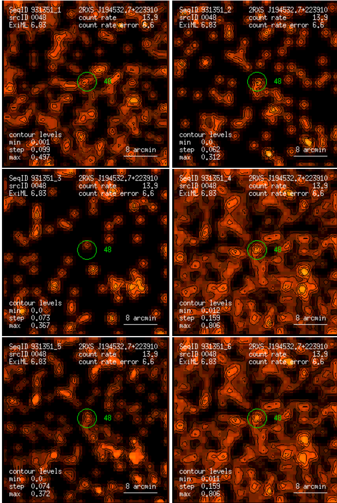
Figure 48: RASS 931351: detection 0048: band rate images, Gaussian filter: (1) PSPC channels 11 – 41, (2) 52 – 90, (3) 91 – 201, (4) 11 – 235, (5) 52 – 201, (6) 11 – 201. Broad band rates in counts/ks. Band rate contour levels in counts/ks/arcmin 2 .
