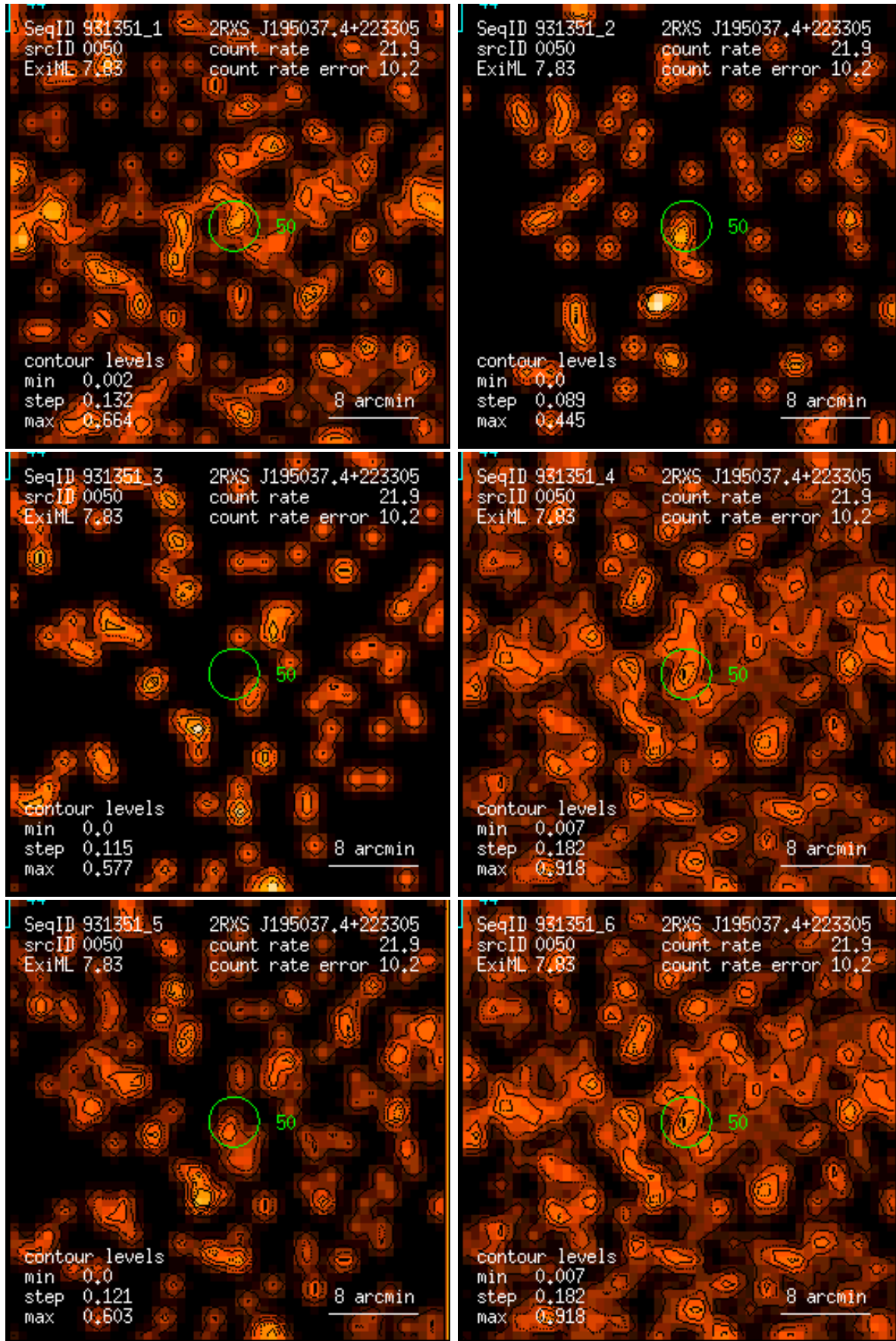
Figure 50: RASS 931351: detection 0050: band rate images, Gaussian filter: (1) PSPC channels 11 – 41, (2) 52 – 90, (3) 91 – 201, (4) 11 – 235, (5) 52 – 201, (6) 11 – 201. Broad band rates in counts/ks. Band rate contour levels in counts/ks/arcmin 2 .
