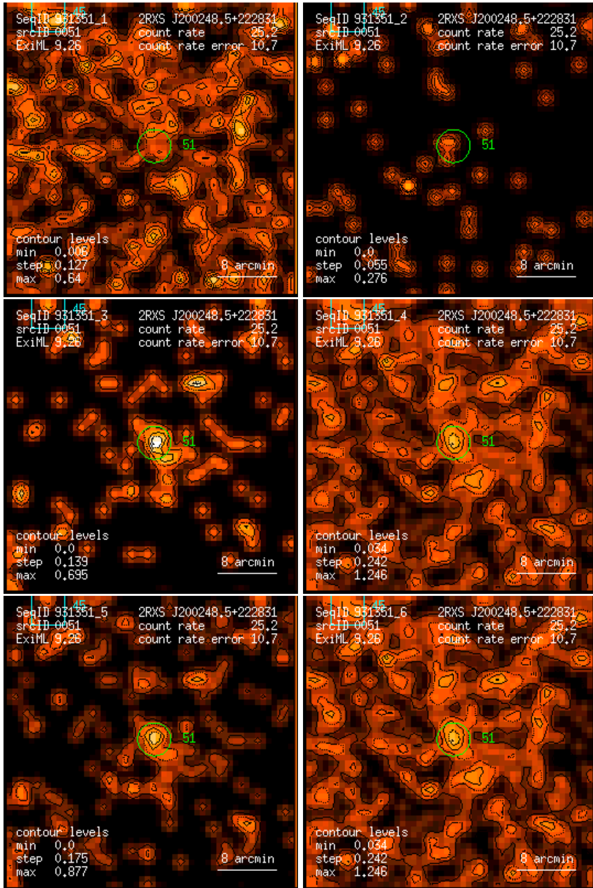
Figure 51: RASS 931351: detection 0051: band rate images, Gaussian filter: (1) PSPC channels 11 – 41, (2) 52 – 90, (3) 91 – 201, (4) 11 – 235, (5) 52 – 201, (6) 11 – 201. Broad band rates in counts/ks. Band rate contour levels in counts/ks/arcmin 2 .
