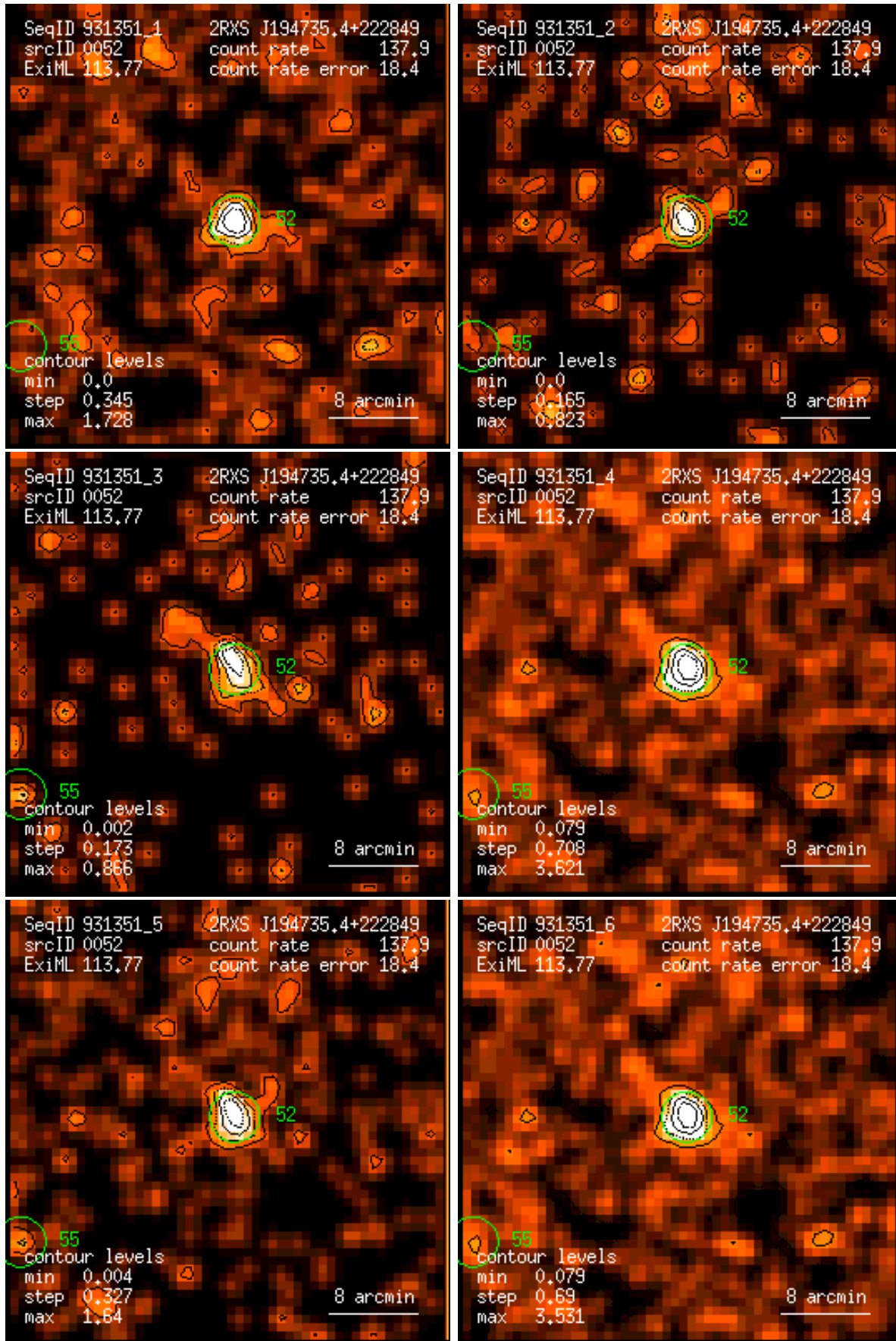
Figure 52: RASS 931351: detection 0052: band rate images, Gaussian filter: (1) PSPC channels 11 – 41, (2) 52 – 90, (3) 91 – 201, (4) 11 – 235, (5) 52 – 201, (6) 11 – 201. Broad band rates in counts/ks. Band rate contour levels in counts/ks/arcmin 2 .
