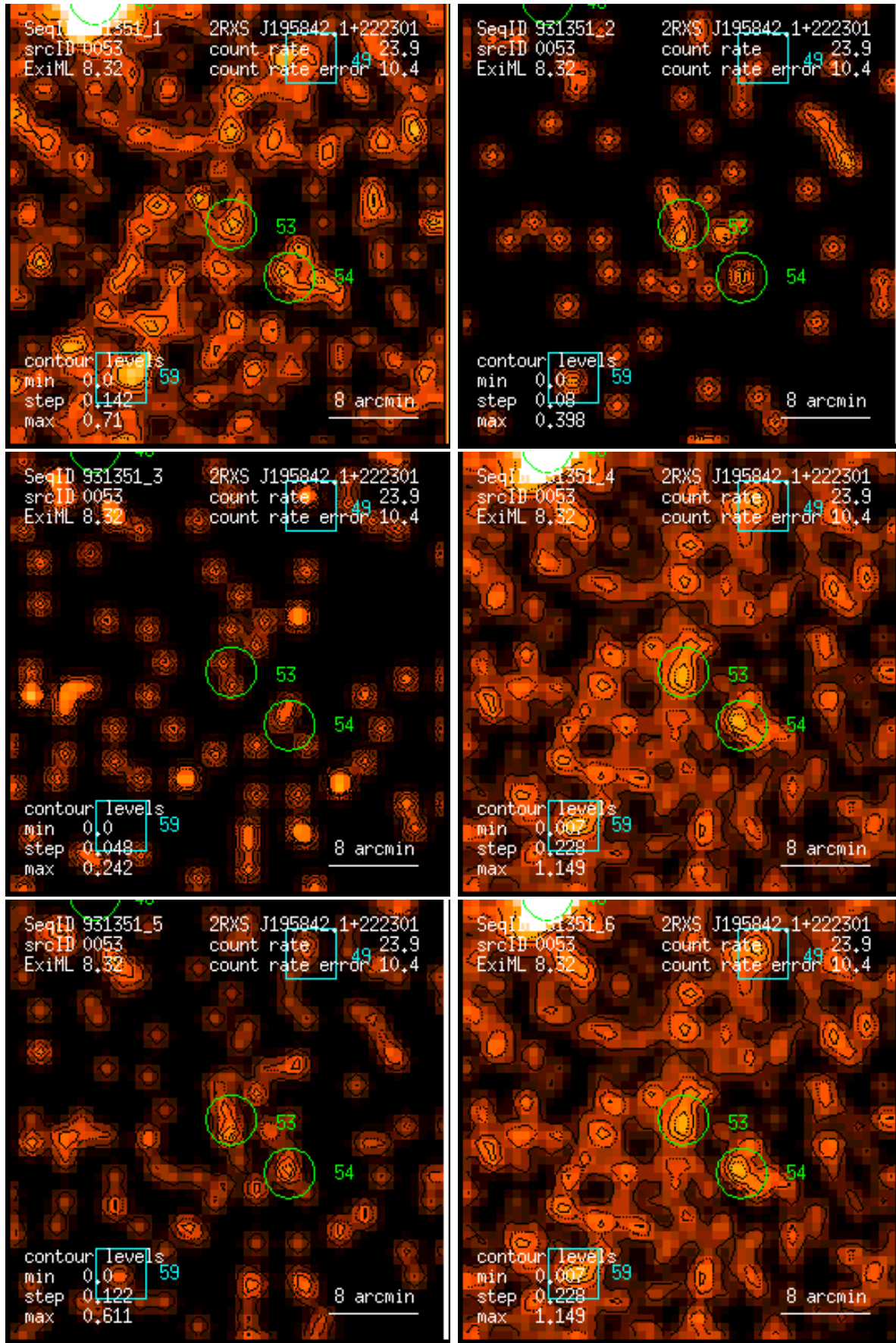
Figure 53: RASS 931351: detection 0053: band rate images, Gaussian filter: (1) PSPC channels 11 – 41, (2) 52 – 90, (3) 91 – 201, (4) 11 – 235, (5) 52 – 201, (6) 11 – 201. Broad band rates in counts/ks. Band rate contour levels in counts/ks/arcmin 2 .
