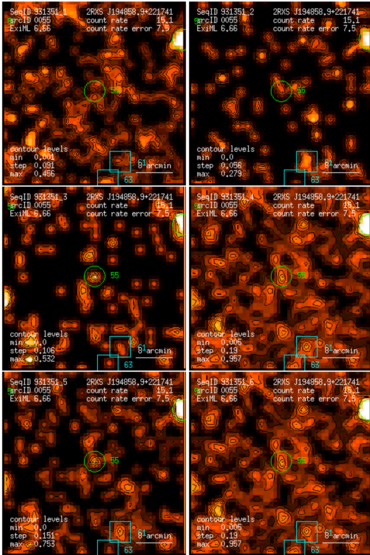
Figure 55: RASS 931351: detection 0055: band rate images, Gaussian filter: (1) PSPC channels 11 – 41, (2) 52 – 90, (3) 91 – 201, (4) 11 – 235, (5) 52 – 201, (6) 11 – 201. Broad band rates in counts/ks. Band rate contour levels in counts/ks/arcmin 2 .
