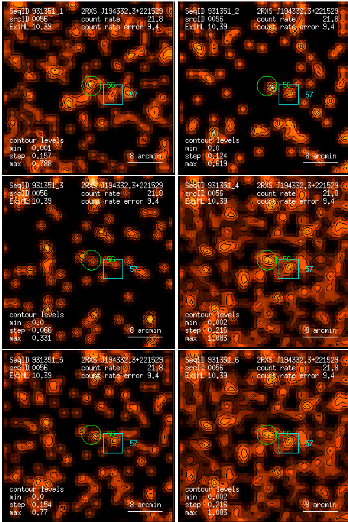
Figure 56: RASS 931351: detection 0056: band rate images, Gaussian filter: (1) PSPC channels 11 – 41, (2) 52 – 90, (3) 91 – 201, (4) 11 – 235, (5) 52 – 201, (6) 11 – 201. Broad band rates in counts/ks. Band rate contour levels in counts/ks/arcmin 2 .
