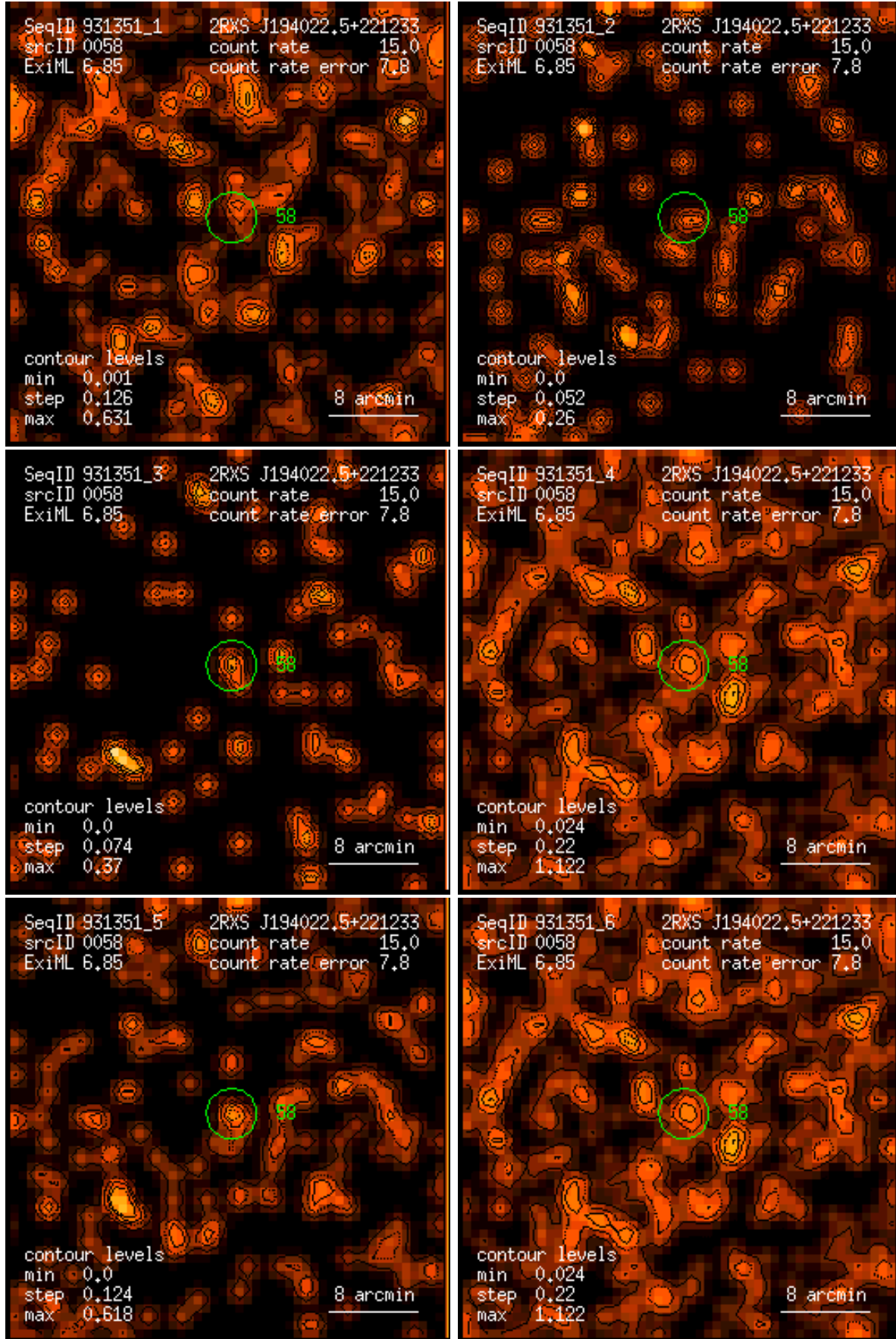
Figure 58: RASS 931351: detection 0058: band rate images, Gaussian filter: (1) PSPC channels 11 – 41, (2) 52 – 90, (3) 91 – 201, (4) 11 – 235, (5) 52 – 201, (6) 11 – 201. Broad band rates in counts/ks. Band rate contour levels in counts/ks/arcmin 2 .
