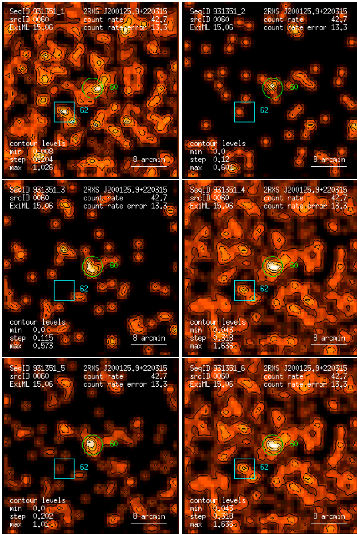
Figure 60: RASS 931351: detection 0060: band rate images, Gaussian filter: (1) PSPC channels 11 – 41, (2) 52 – 90, (3) 91 – 201, (4) 11 – 235, (5) 52 – 201, (6) 11 – 201. Broad band rates in counts/ks. Band rate contour levels in counts/ks/arcmin 2 .
