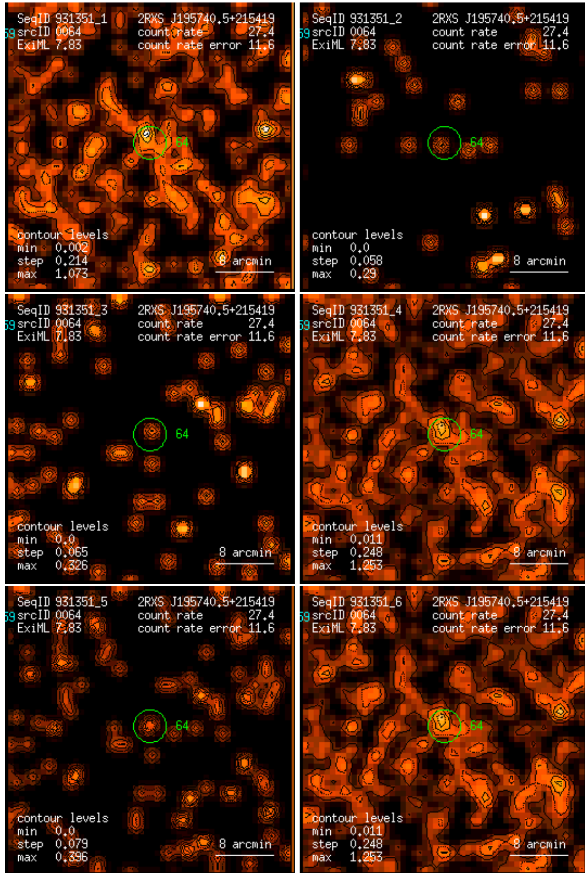
Figure 64: RASS 931351: detection 0064: band rate images, Gaussian filter: (1) PSPC channels 11 – 41, (2) 52 – 90, (3) 91 – 201, (4) 11 – 235, (5) 52 – 201, (6) 11 – 201. Broad band rates in counts/ks. Band rate contour levels in counts/ks/arcmin 2 .
