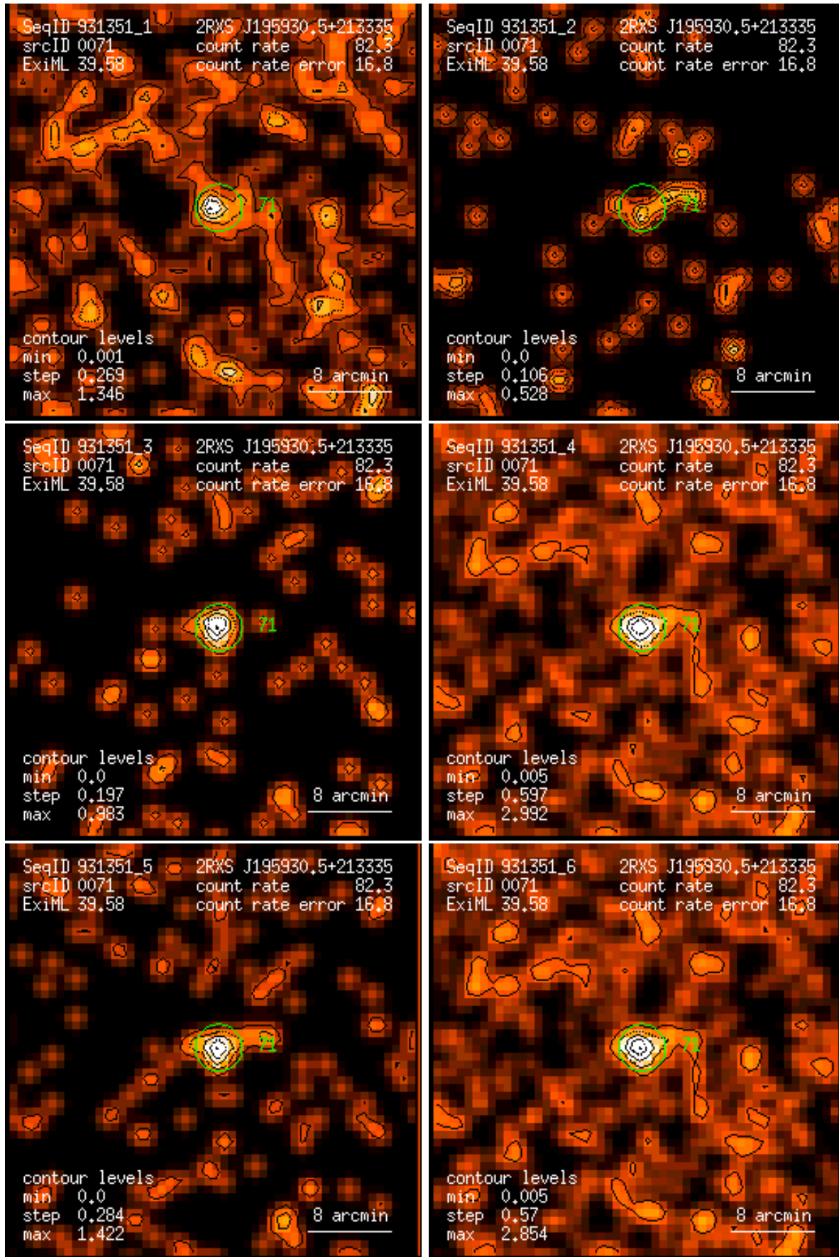
Figure 71: RASS 931351: detection 0071: band rate images, Gaussian filter: (1) PSPC channels 11 – 41, (2) 52 – 90, (3) 91 – 201, (4) 11 – 235, (5) 52 – 201, (6) 11 – 201. Broad band rates in counts/ks. Band rate contour levels in counts/ks/arcmin 2 .
