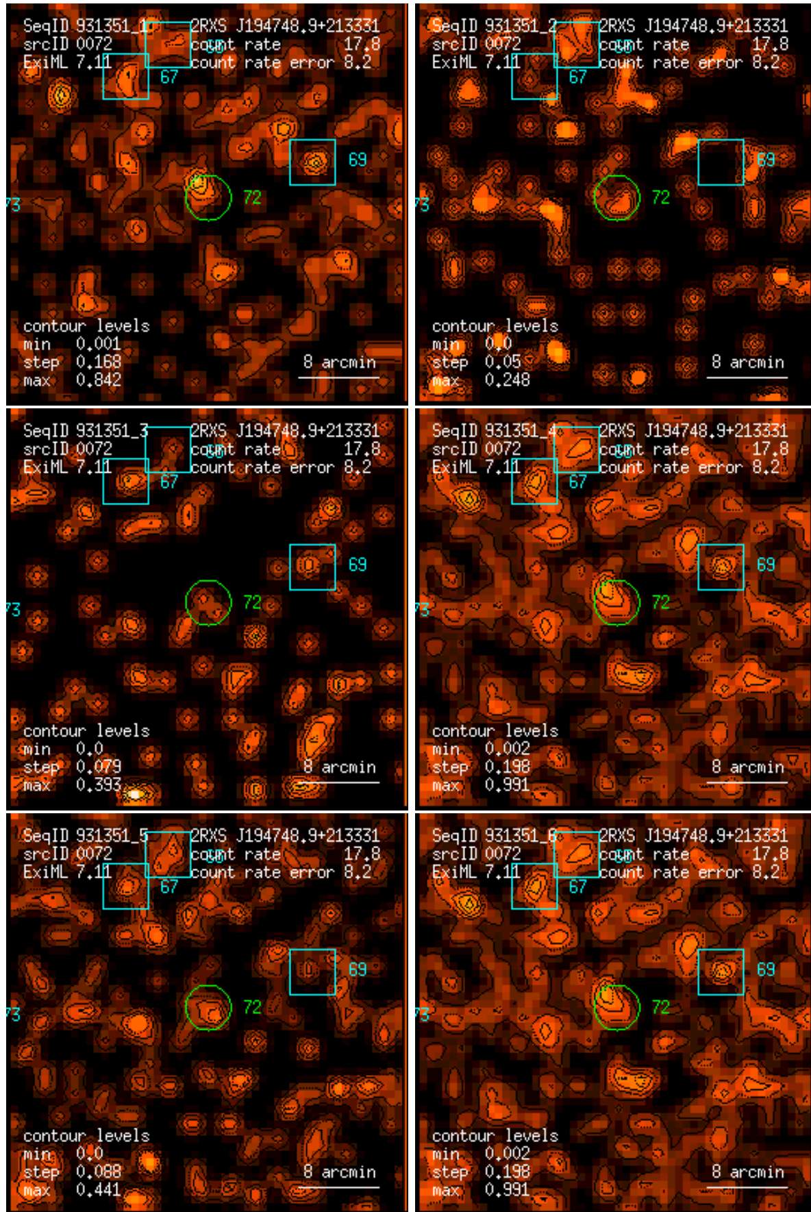
Figure 72: RASS 931351: detection 0072: band rate images, Gaussian filter: (1) PSPC channels 11 – 41, (2) 52 – 90, (3) 91 – 201, (4) 11 – 235, (5) 52 – 201, (6) 11 – 201. Broad band rates in counts/ks. Band rate contour levels in counts/ks/arcmin 2 .
