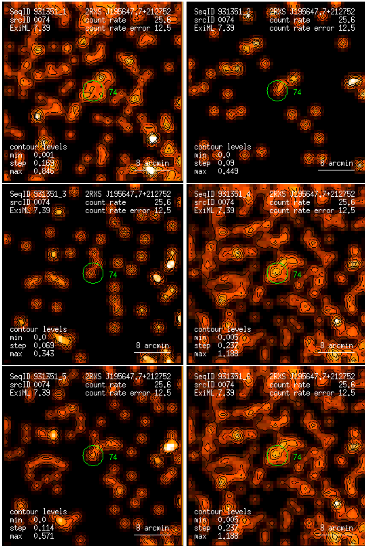
Figure 74: RASS 931351: detection 0074: band rate images, Gaussian filter: (1) PSPC channels 11 – 41, (2) 52 – 90, (3) 91 – 201, (4) 11 – 235, (5) 52 – 201, (6) 11 – 201. Broad band rates in counts/ks. Band rate contour levels in counts/ks/arcmin 2 .
