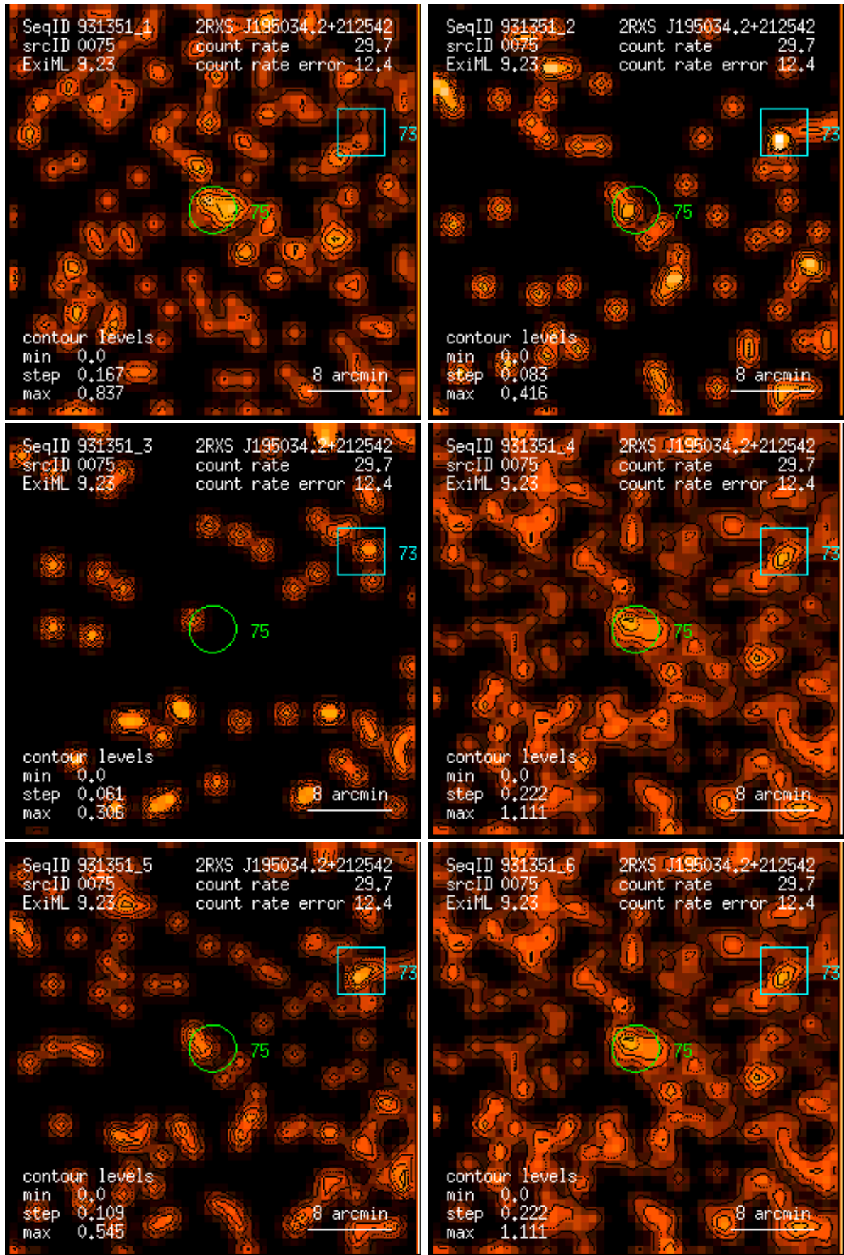
Figure 75: RASS 931351: detection 0075: band rate images, Gaussian filter: (1) PSPC channels 11 – 41, (2) 52 – 90, (3) 91 – 201, (4) 11 – 235, (5) 52 – 201, (6) 11 – 201. Broad band rates in counts/ks. Band rate contour levels in counts/ks/arcmin 2 .
