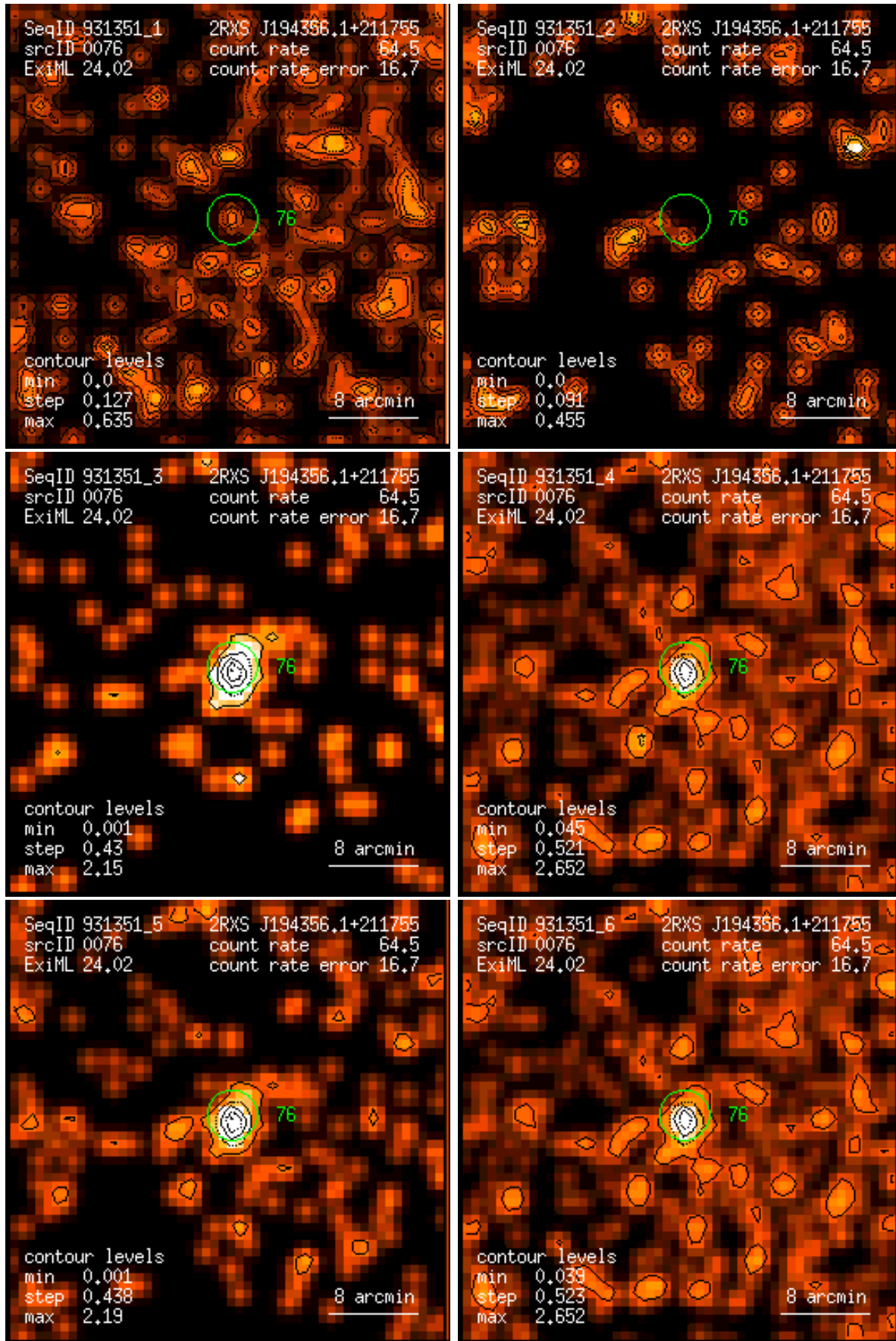
Figure 76: RASS 931351: detection 0076: band rate images, Gaussian filter: (1) PSPC channels 11 – 41, (2) 52 – 90, (3) 91 – 201, (4) 11 – 235, (5) 52 – 201, (6) 11 – 201. Broad band rates in counts/ks. Band rate contour levels in counts/ks/arcmin 2 .
