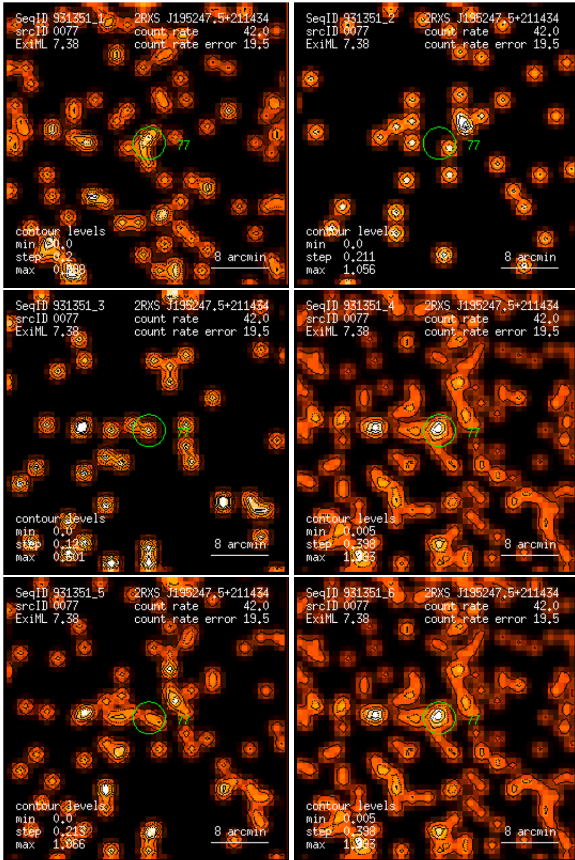
Figure 77: RASS 931351: detection 0077: band rate images, Gaussian filter: (1) PSPC channels 11 – 41, (2) 52 – 90, (3) 91 – 201, (4) 11 – 235, (5) 52 – 201, (6) 11 – 201. Broad band rates in counts/ks. Band rate contour levels in counts/ks/arcmin 2 .
