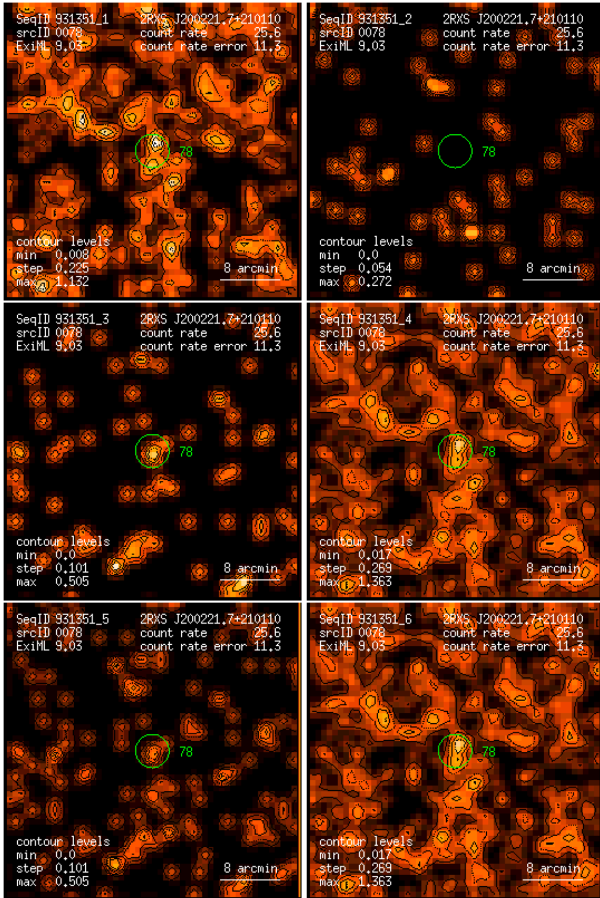
Figure 78: RASS 931351: detection 0078: band rate images, Gaussian filter: (1) PSPC channels 11 – 41, (2) 52 – 90, (3) 91 – 201, (4) 11 – 235, (5) 52 – 201, (6) 11 – 201. Broad band rates in counts/ks. Band rate contour levels in counts/ks/arcmin 2 .
