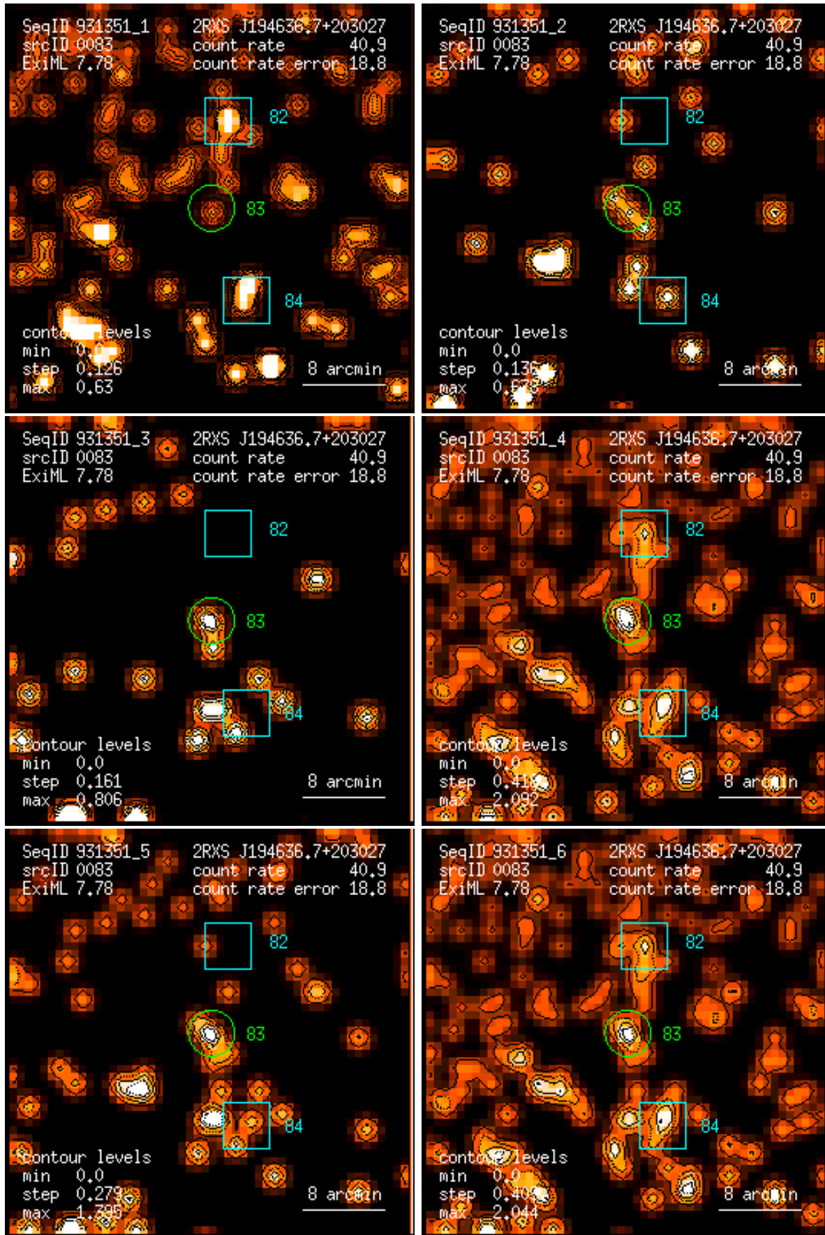
Figure 83: RASS 931351: detection 0083: band rate images, Gaussian filter: (1) PSPC channels 11 – 41, (2) 52 – 90, (3) 91 – 201, (4) 11 – 235, (5) 52 – 201, (6) 11 – 201. Broad band rates in counts/ks. Band rate contour levels in counts/ks/arcmin 2 .
