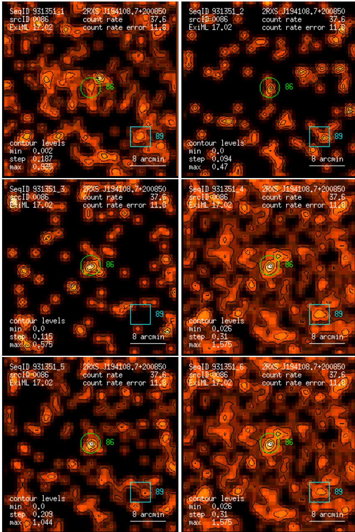
Figure 86: RASS 931351: detection 0086: band rate images, Gaussian filter: (1) PSPC channels 11 – 41, (2) 52 – 90, (3) 91 – 201, (4) 11 – 235, (5) 52 – 201, (6) 11 – 201. Broad band rates in counts/ks. Band rate contour levels in counts/ks/arcmin 2 .
