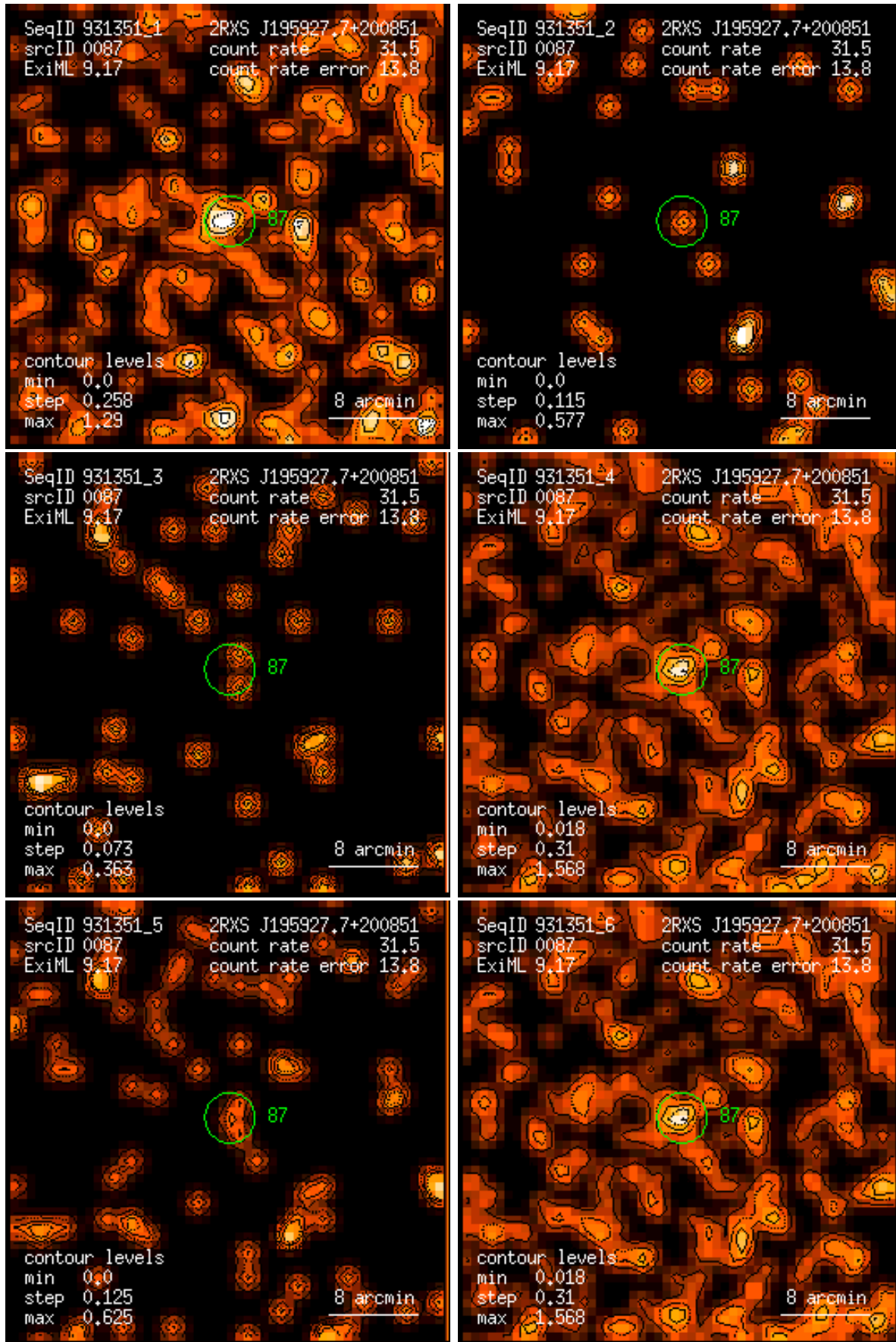
Figure 87: RASS 931351: detection 0087: band rate images, Gaussian filter: (1) PSPC channels 11 – 41, (2) 52 – 90, (3) 91 – 201, (4) 11 – 235, (5) 52 – 201, (6) 11 – 201. Broad band rates in counts/ks. Band rate contour levels in counts/ks/arcmin 2 .
