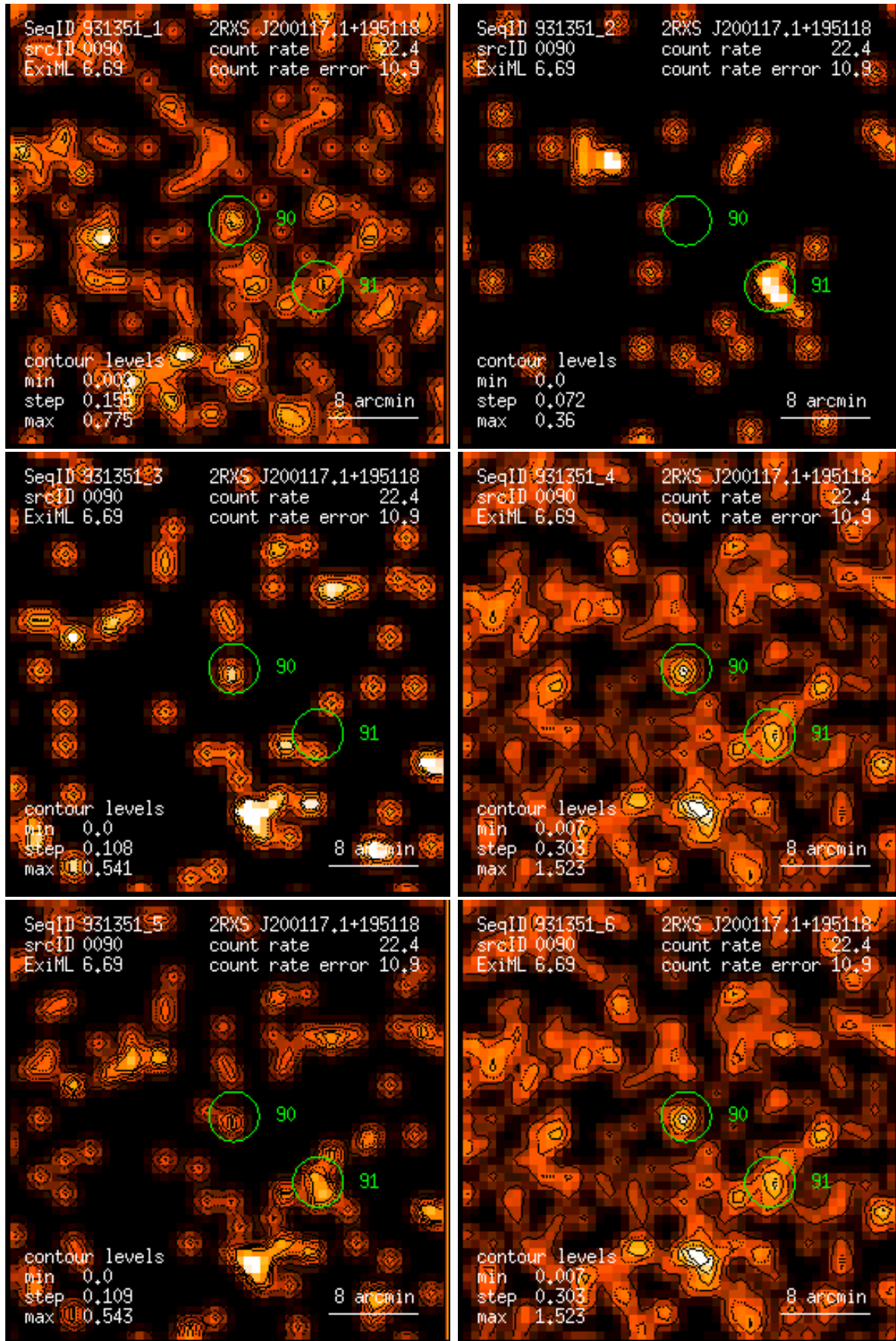
Figure 90: RASS 931351: detection 0090: band rate images, Gaussian filter: (1) PSPC channels 11 – 41, (2) 52 – 90, (3) 91 – 201, (4) 11 – 235, (5) 52 – 201, (6) 11 – 201. Broad band rates in counts/ks. Band rate contour levels in counts/ks/arcmin 2 .
