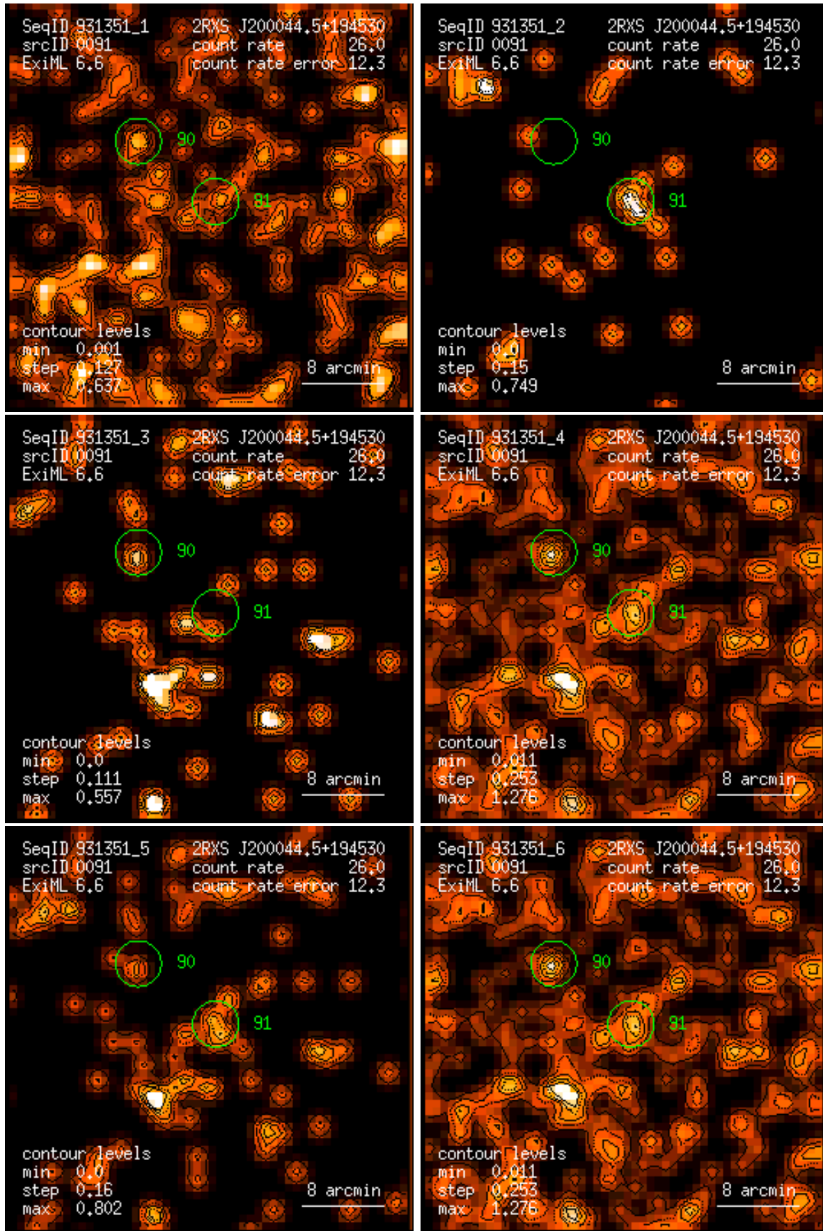
Figure 91: RASS 931351: detection 0091: band rate images, Gaussian filter: (1) PSPC channels 11 – 41, (2) 52 – 90, (3) 91 – 201, (4) 11 – 235, (5) 52 – 201, (6) 11 – 201. Broad band rates in counts/ks. Band rate contour levels in counts/ks/arcmin 2 .
