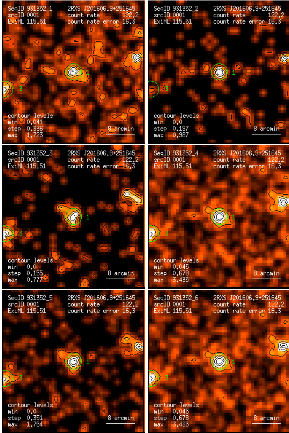
Figure 1: RASS 931352: detection 0001: band rate images, Gaussian filter: (1) PSPC channels 11 – 41, (2) 52 – 90, (3) 91 – 201, (4) 11 – 235, (5) 52 – 201, (6) 11 – 201. Broad band rates in counts/ks. Band rate contour levels in counts/ks/arcmin 2 .
