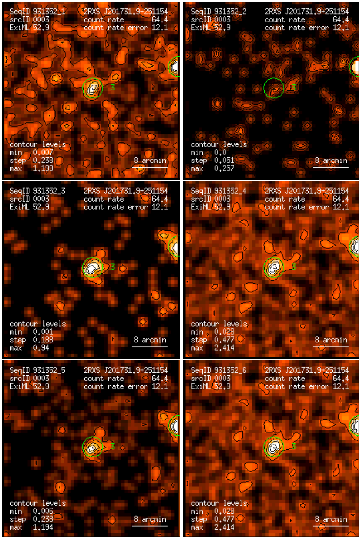
Figure 3: RASS 931352: detection 0003: band rate images, Gaussian filter: (1) PSPC channels 11 – 41, (2) 52 – 90, (3) 91 – 201, (4) 11 – 235, (5) 52 – 201, (6) 11 – 201. Broad band rates in counts/ks. Band rate contour levels in counts/ks/arcmin 2 .
