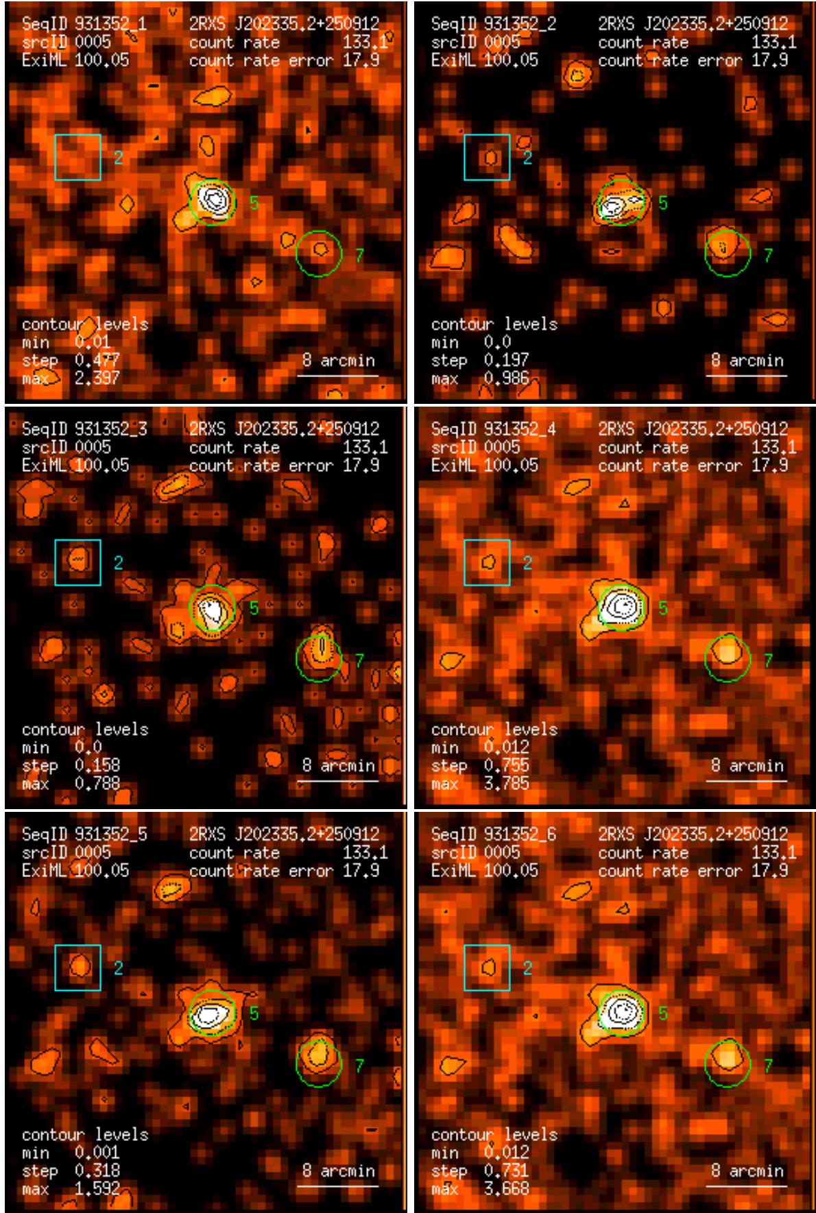
Figure 5: RASS 931352: detection 0005: band rate images, Gaussian filter: (1) PSPC channels 11 – 41, (2) 52 – 90, (3) 91 – 201, (4) 11 – 235, (5) 52 – 201, (6) 11 – 201. Broad band rates in counts/ks. Band rate contour levels in counts/ks/arcmin 2 .
