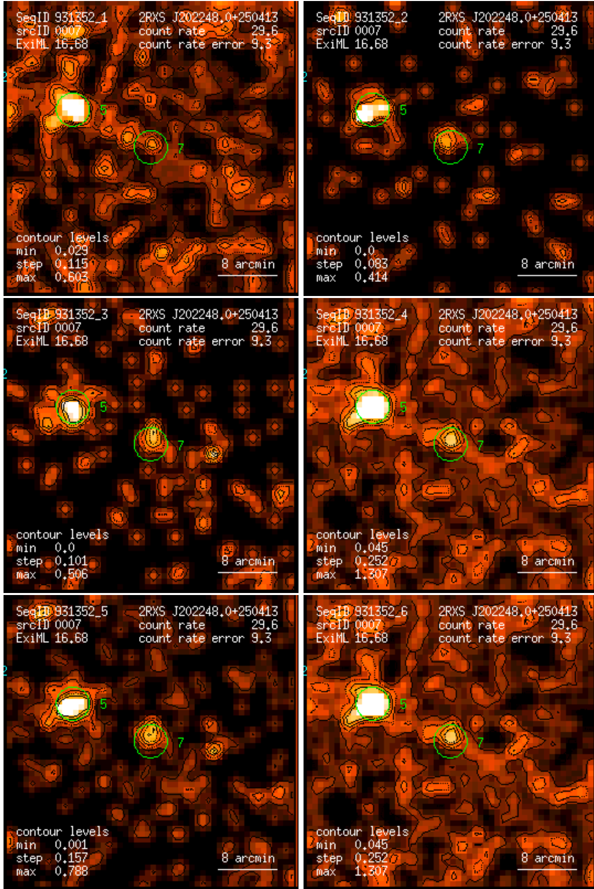
Figure 7: RASS 931352: detection 0007: band rate images, Gaussian filter: (1) PSPC channels 11 – 41, (2) 52 – 90, (3) 91 – 201, (4) 11 – 235, (5) 52 – 201, (6) 11 – 201. Broad band rates in counts/ks. Band rate contour levels in counts/ks/arcmin 2 .
