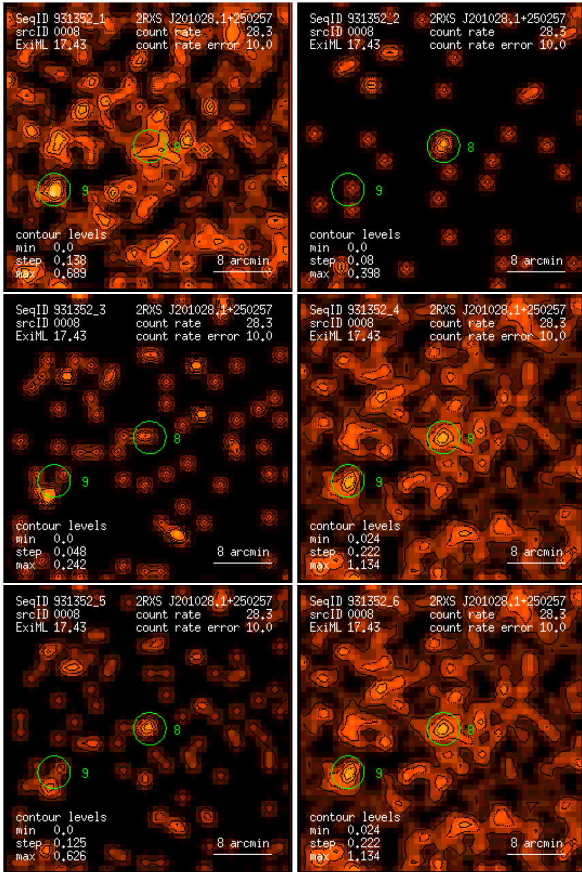
Figure 8: RASS 931352: detection 0008: band rate images, Gaussian filter: (1) PSPC channels 11 – 41, (2) 52 – 90, (3) 91 – 201, (4) 11 – 235, (5) 52 – 201, (6) 11 – 201. Broad band rates in counts/ks. Band rate contour levels in counts/ks/arcmin 2 .
