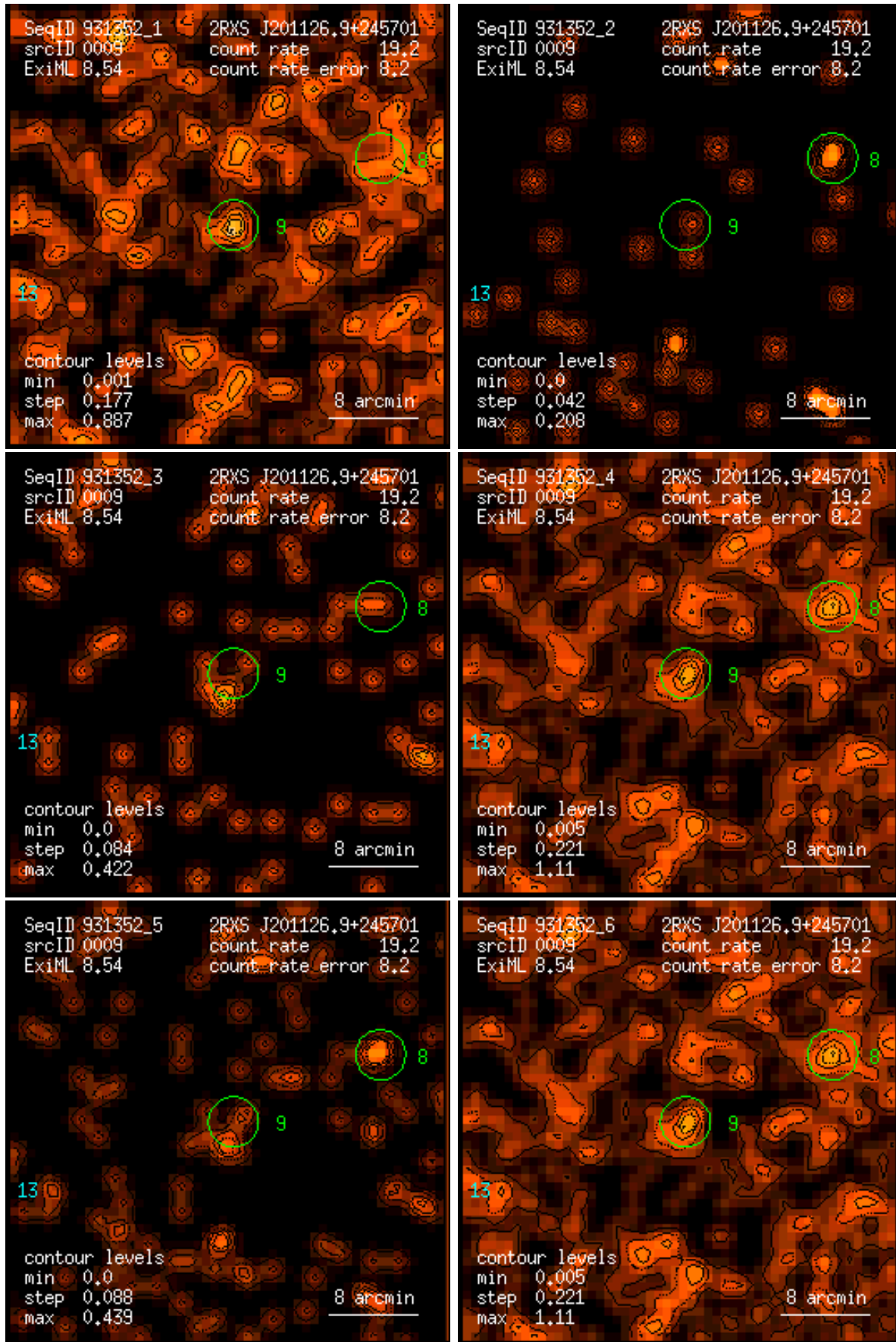
Figure 9: RASS 931352: detection 0009: band rate images, Gaussian filter: (1) PSPC channels 11 – 41, (2) 52 – 90, (3) 91 – 201, (4) 11 – 235, (5) 52 – 201, (6) 11 – 201. Broad band rates in counts/ks. Band rate contour levels in counts/ks/arcmin 2 .
