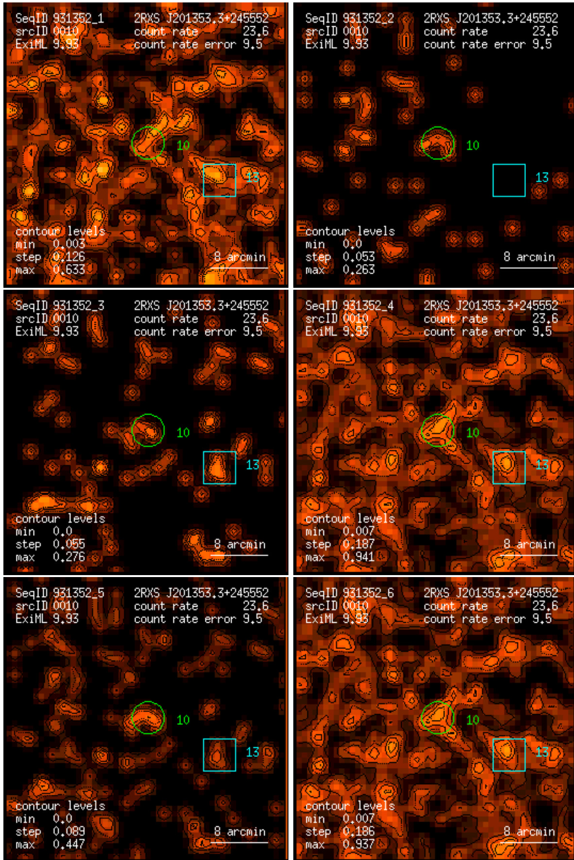
Figure 10: RASS 931352: detection 0010: band rate images, Gaussian filter: (1) PSPC channels 11 – 41, (2) 52 – 90, (3) 91 – 201, (4) 11 – 235, (5) 52 – 201, (6) 11 – 201. Broad band rates in counts/ks. Band rate contour levels in counts/ks/arcmin 2 .
