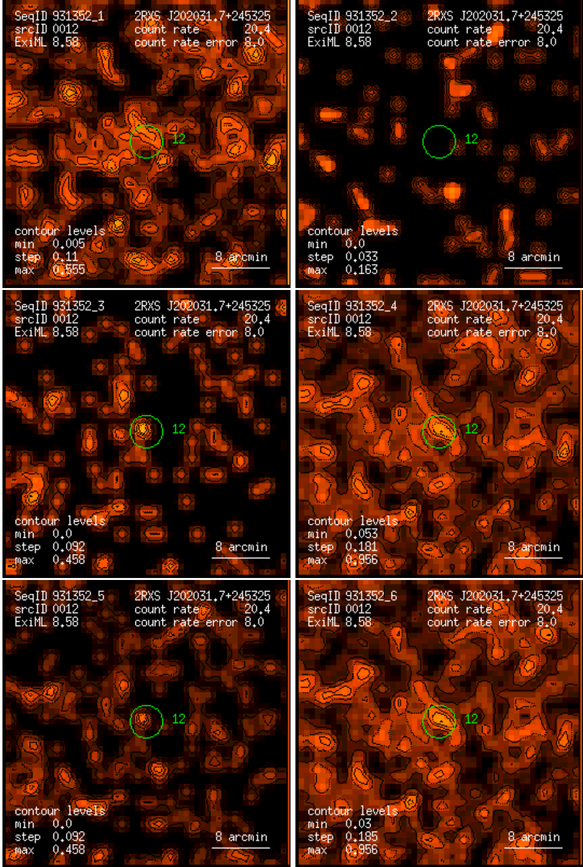
Figure 12: RASS 931352: detection 0012: band rate images, Gaussian filter: (1) PSPC channels 11 – 41, (2) 52 – 90, (3) 91 – 201, (4) 11 – 235, (5) 52 – 201, (6) 11 – 201. Broad band rates in counts/ks. Band rate contour levels in counts/ks/arcmin 2 .
