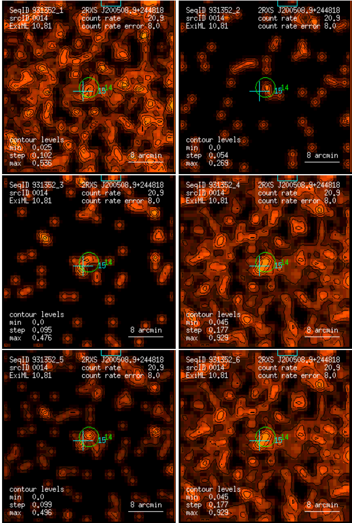
Figure 14: RASS 931352: detection 0014: band rate images, Gaussian filter: (1) PSPC channels 11 – 41, (2) 52 – 90, (3) 91 – 201, (4) 11 – 235, (5) 52 – 201, (6) 11 – 201. Broad band rates in counts/ks. Band rate contour levels in counts/ks/arcmin 2 .
