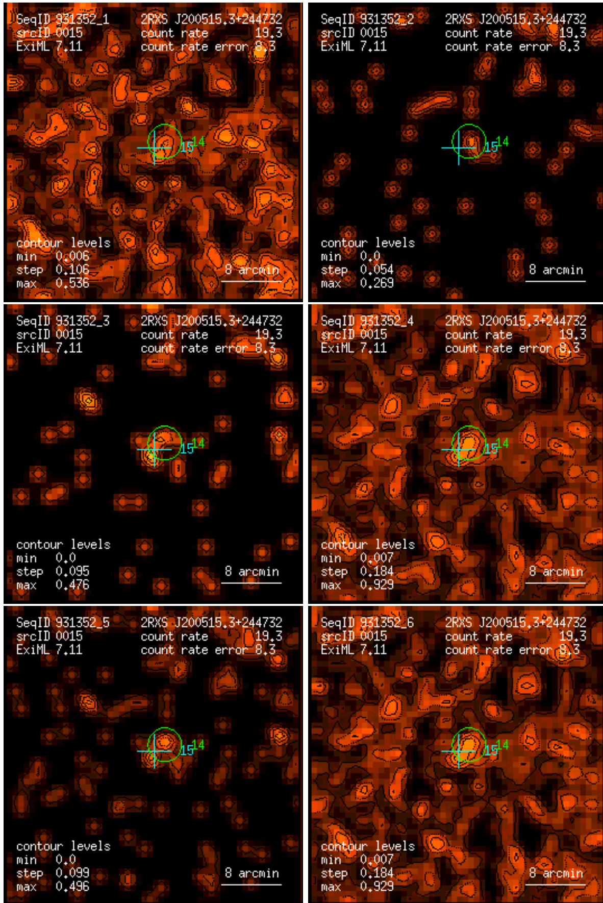
Figure 15: RASS 931352: detection 0015: band rate images, Gaussian filter: (1) PSPC channels 11 – 41, (2) 52 – 90, (3) 91 – 201, (4) 11 – 235, (5) 52 – 201, (6) 11 – 201. Broad band rates in counts/ks. Band rate contour levels in counts/ks/arcmin 2 .
