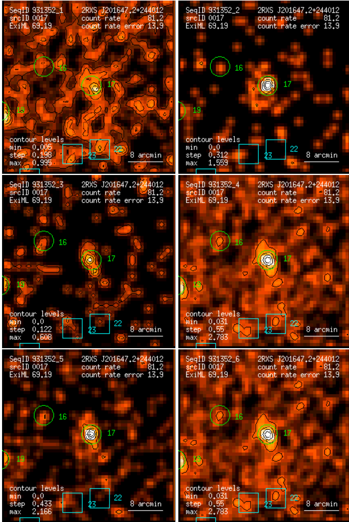
Figure 17: RASS 931352: detection 0017: band rate images, Gaussian filter: (1) PSPC channels 11 – 41, (2) 52 – 90, (3) 91 – 201, (4) 11 – 235, (5) 52 – 201, (6) 11 – 201. Broad band rates in counts/ks. Band rate contour levels in counts/ks/arcmin 2 .
