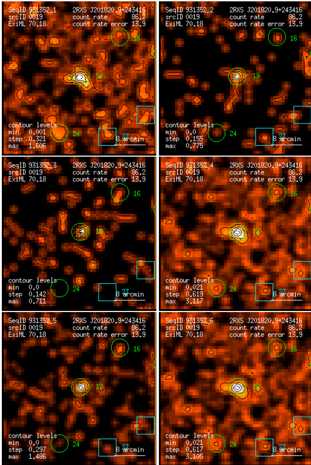
Figure 19: RASS 931352: detection 0019: band rate images, Gaussian filter: (1) PSPC channels 11 – 41, (2) 52 – 90, (3) 91 – 201, (4) 11 – 235, (5) 52 – 201, (6) 11 – 201. Broad band rates in counts/ks. Band rate contour levels in counts/ks/arcmin 2 .
