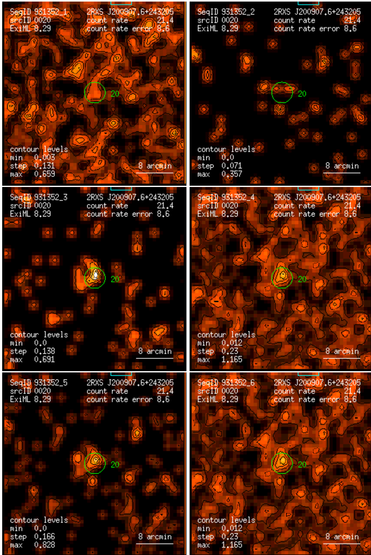
Figure 20: RASS 931352: detection 0020: band rate images, Gaussian filter: (1) PSPC channels 11 – 41, (2) 52 – 90, (3) 91 – 201, (4) 11 – 235, (5) 52 – 201, (6) 11 – 201. Broad band rates in counts/ks. Band rate contour levels in counts/ks/arcmin 2 .
