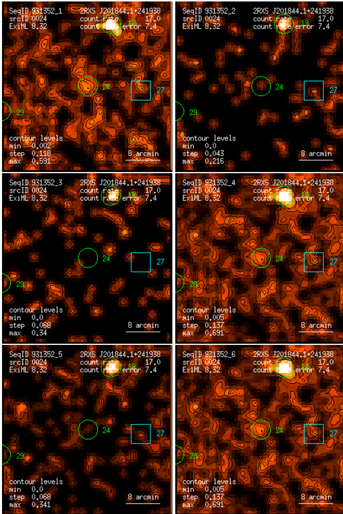
Figure 24: RASS 931352: detection 0024: band rate images, Gaussian filter: (1) PSPC channels 11 – 41, (2) 52 – 90, (3) 91 – 201, (4) 11 – 235, (5) 52 – 201, (6) 11 – 201. Broad band rates in counts/ks. Band rate contour levels in counts/ks/arcmin 2 .
