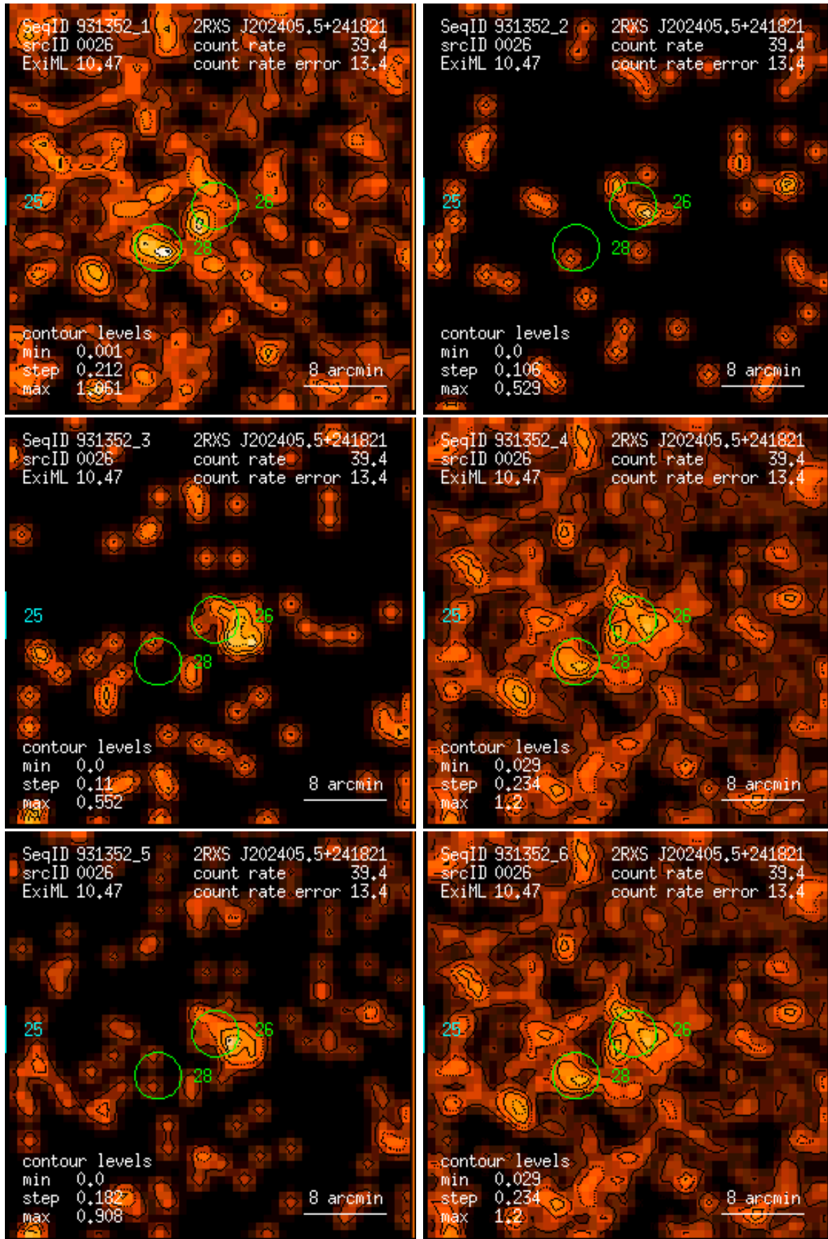
Figure 26: RASS 931352: detection 0026: band rate images, Gaussian filter: (1) PSPC channels 11 – 41, (2) 52 – 90, (3) 91 – 201, (4) 11 – 235, (5) 52 – 201, (6) 11 – 201. Broad band rates in counts/ks. Band rate contour levels in counts/ks/arcmin 2 .
